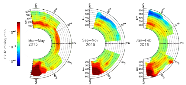
Figure 1: Example of C_2H_2 volume mixing ratio maps from 120 to 600 km between March 2015 and February 2016.
