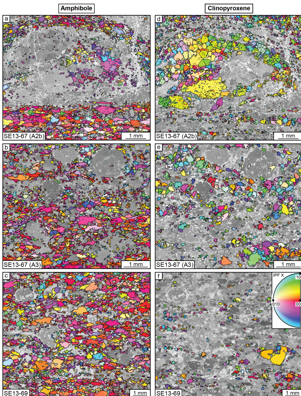
Figure 9. X direction inverse pole figure (IPF) coloring orientation maps for (a–c) amphibole and (d–f) clinopyroxene.
