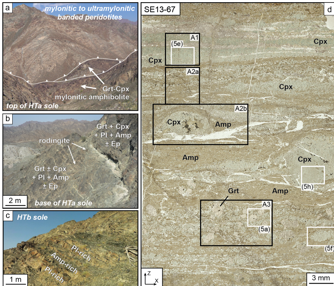
Figure 2. Photographs of the base of the Semail ophiolite outcropping in the Sumeini region (modified after Soret et al., 2017). (a) Basal contact between banded peridotite and the Grt–Cpx amphibolite of the metamorphic sole (zone HTa); (b) base of the HTa unit, widely affected by Ca-rich metasomatism (rodingitization); (c) layered structure in zone HTb with alternations from plagioclase-rich to darker amphibole-rich layers; (d–h) well-preserved mineral equilibrium texture and deformation structure from peak conditions in the HTa amphibolite at Sumeini (~2.5 m from the contact). Black boxes refer to EBSD maps shown in Figs. 3 and 4. White boxes correspond to photographs in Fig. 5.
