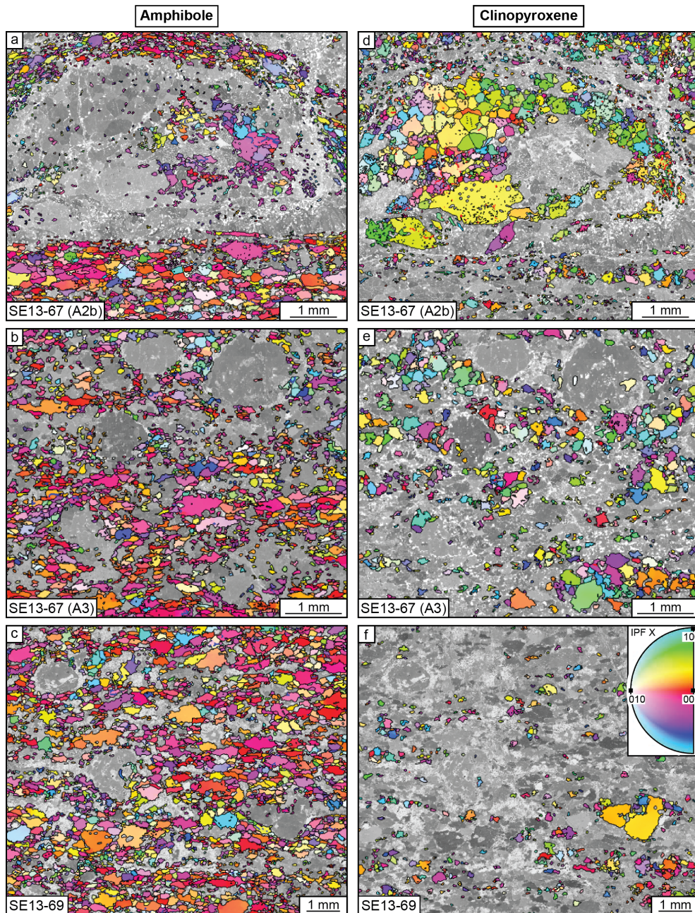
Figure 9. X direction inverse pole figure (IPF) coloring orientation maps for (a–c) amphibole and (d–f) clinopyroxene.
