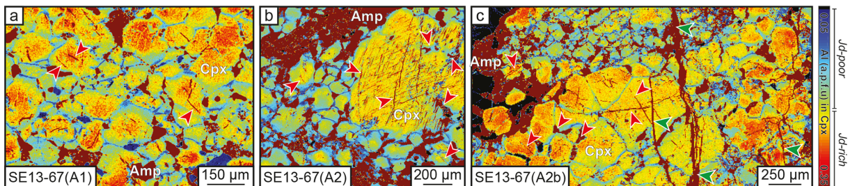
Figure 7. (a) Compositional map of Al of clinopyroxene in mono- and polymineralic layers of sample SE13-67. Red arrows point to amphibole in clinopyroxene microfractures or in interstitial positions at new clinopyroxene boundaries; Jd: jadeite content; see the text for details.
