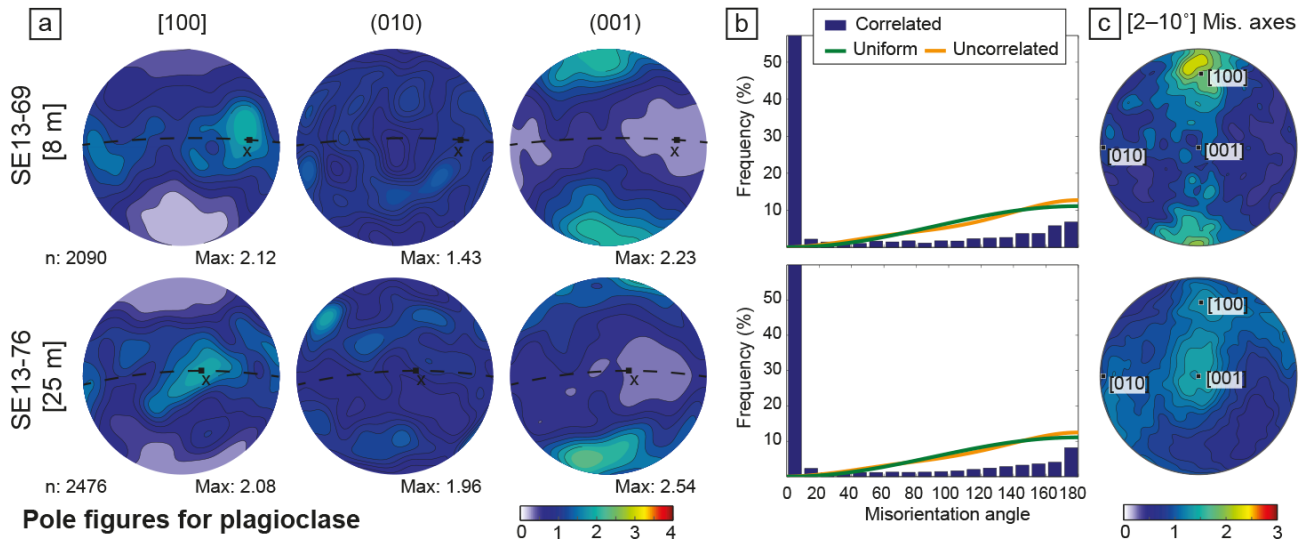
Figure 12. (a) Pole figures illustrating CPO of plagioclase in samples from the HTa unit of Sumeini; (b) distribution of misorientation angles; (c) inverse pole figures showing the distribution of correlated misorientation axes (between 2 and 10°). See caption of Fig. 7 for details.
