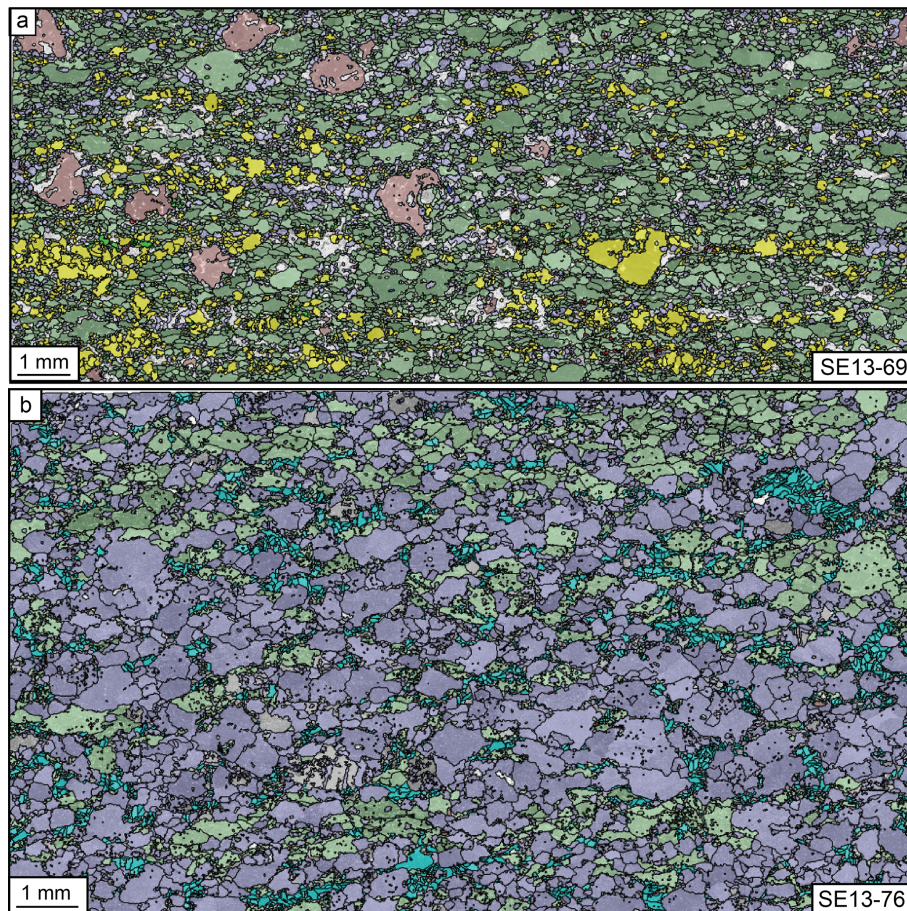
Figure 4. EBSD phase maps (a) from a slightly retrogressed, at amphibolite facies, garnet–clinopyroxene-bearing amphibolite at the top of HTa unit (sample SE13-69; Sumeini area); (b) from a highly retrogressed garnet–clinopyroxene-free amphibolite at the base of HTa unit (sample SE13-76; Sumeini area).
