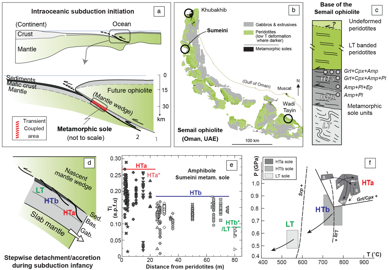
Figure 1. (a) Geodynamic setting of metamorphic sole formation during intraoceanic subduction infancy (modified after Agard et al., 2016); (b) simplified geological map of the Semail ophiolite, highlighting the outcrops of metamorphic sole beneath the ophiolite mantle (modified after Nicolas et al., 2000); (c) schematic log of the base of the Oman ophiolite showing the structural position of the samples from Khubakhib (K), Sumeini (S) and Wadi Tayin (WT). See Table 1 for details; (d) close-up view of the tectonic configuration along the nascent plate interface, during the formation and exhumation of the HTa, HTb and LT soles until reaching the steady state (sketch modified after Agard et al., 2016, and Soret et al., 2017); s: sediment, b: basalt, g: gabbro, m: mantle peridotite; (e) amphibole Ti vs. Si content in amphibolite samples from Sumeini (after Soret et al., 2017) outlining the discontinuous decrease in T conditions during the exhumation of the HT metamorphic sole; (f) compilations of P – T estimates and associated P – T paths (after Soret et al., 2017) from the Grt–Cpx amphibolite (HTa) to the Pl-rich amphibolite (HTb) and greenschist facies (LT) metamorphic sole units.
