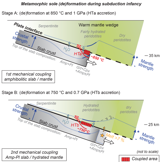
Figure 14. Schematic view of the strength evolution in the top of the slab crust and in the peridotite across the nascent subduction interface. Strong and transient interplate mechanical coupling allows the detachment and accretion of HTa and HTb metamorphic sole units to the peridotite (of the future ophiolite).
