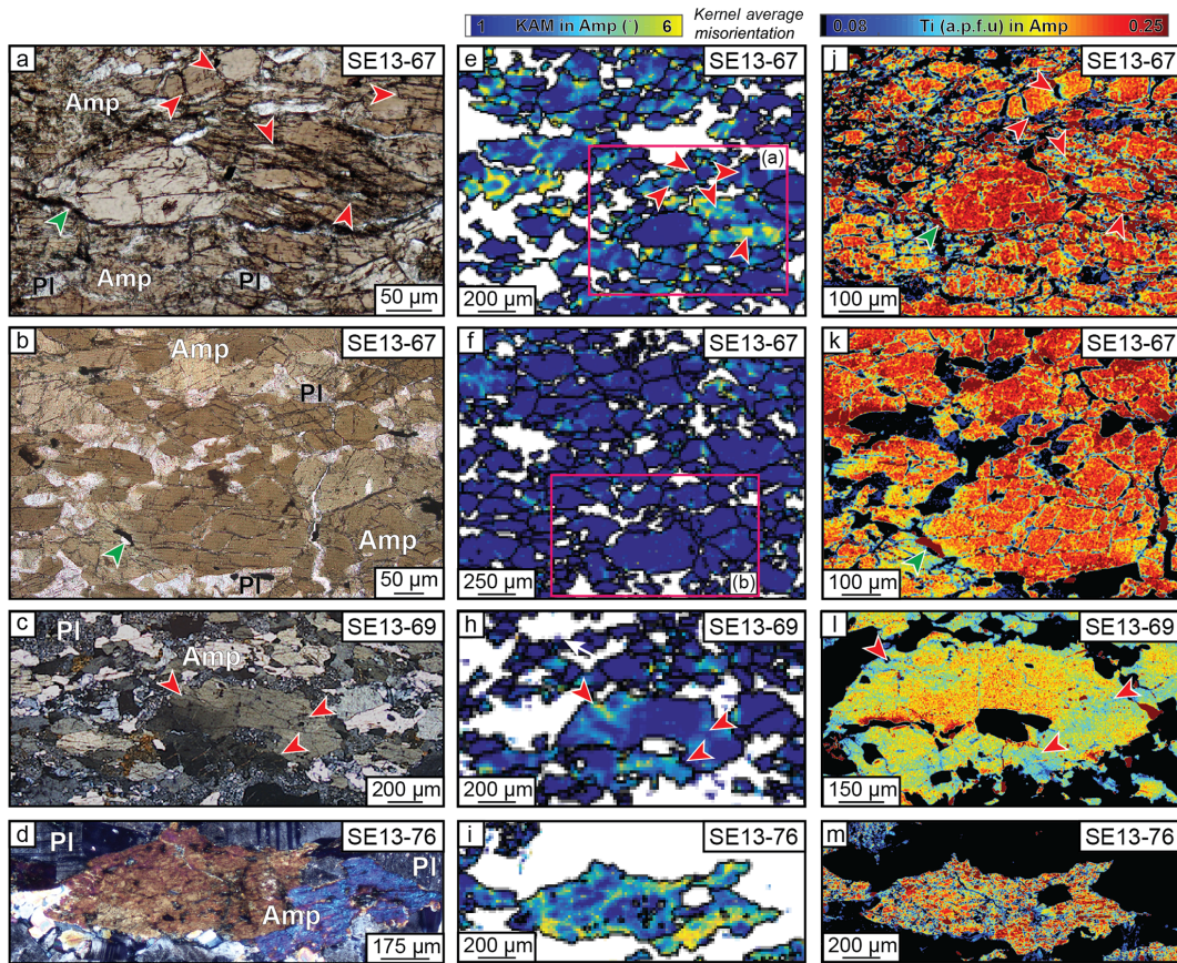
Figure 6. (a–d) Photographs of representative textures of amphibole, (e, f, h, i) (2–10°) intracrystalline misorientation (to the mean grain orientation) and (j–m) compositional map of Ti of amphibole in samples sorted as a function of the distance from the peridotite. Red and green arrows point to amphibole microfractures and ilmenite veinlets or crystals, respectively.
