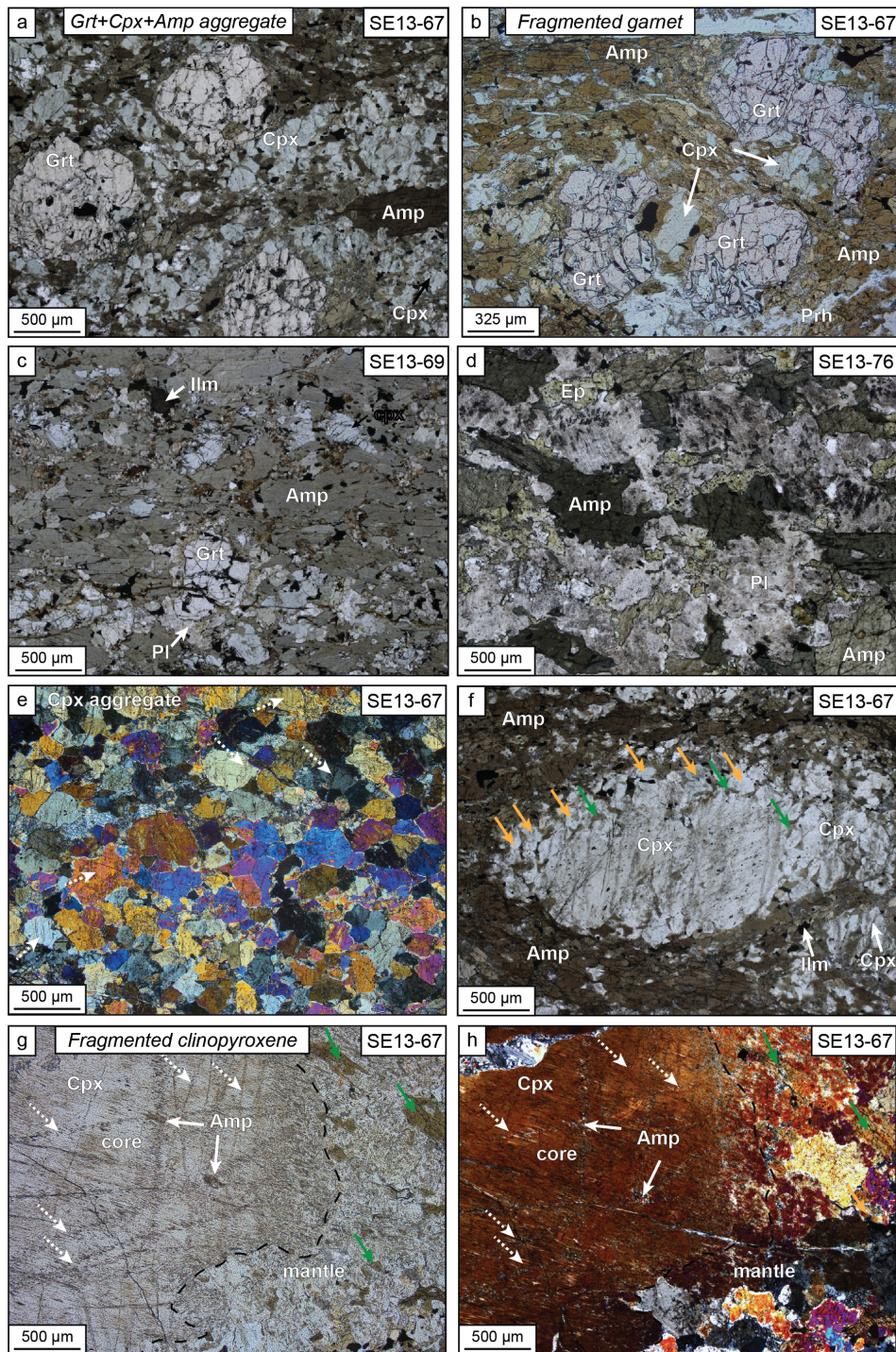
Figure 5. Photographs of representative microstructures in the HTa amphibolites. (a) Garnet porphyroclasts surrounded by a fine-grained matrix of Cpx + Amp (Area 3); (b) fractured garnet porphyroclast with fractures filled by a fine-grained matrix composed of Cpx + Amp; (c) ~ 8 m from the contact, showing greater retrogression characterized by an increase in plagioclase and brown amphibole at the expense of Grt + Cpx; (d) ~ 25 m from the contact (base of HTa), highly retrogressed amphibolite associated with secondary crystallization of coarse-grained brown-to-green amphibole, epidote and plagioclase; (e) monomineralic layer of recrystallized clinopyroxene by subgrain rotation; (f) sheared Cpx porphyroclast wrapped by fine-grained brown Amp (Area 2); (g) and (h; cross polarized light) core-and-mantle structure in a Cpx porphyroclast with and minute amphibole in sealed microfractures (fluid inclusions trails) and at grain boundaries of the porphyroclast mantle. Orange and green arrows point to small new clinopyroxene deriving from the fragmented clinopyroxene porphyroclast and secondary amphibole, respectively. See details in the text.
