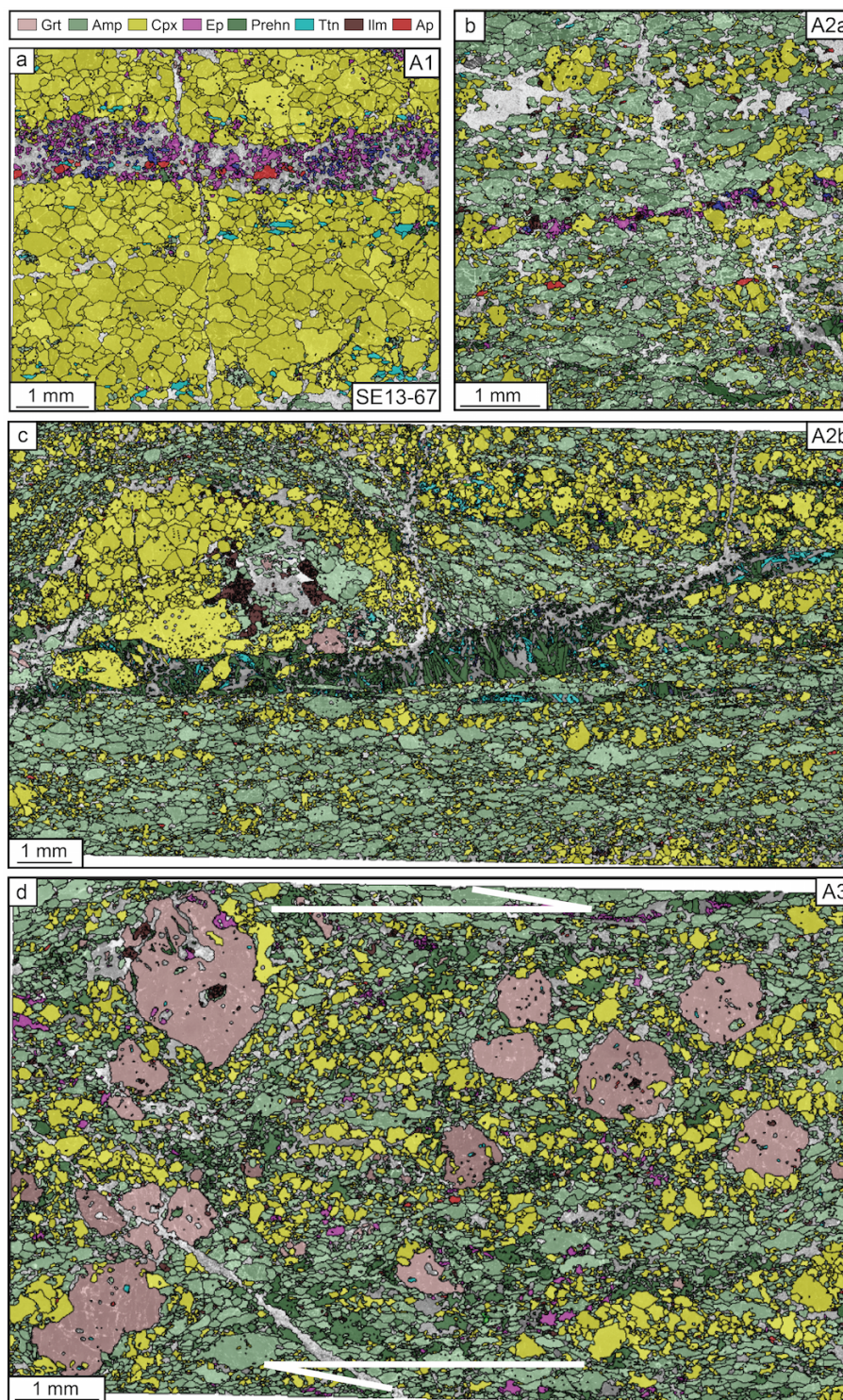
Figure 3. EBSD phase maps from a Grt–Cpx-bearing amphibolite sampled at \sim 2.5 m from the contact with peridotite (sample SE13-67) and showing the best-preserved microstructures. (a) Area 1 (A1) composed essentially of clinopyroxene with a late vein of epidote; (b) and (c) Area 2 (A2) composed of amphibole and clinopyroxene. (c) A late prehnite vein crosscuts the sample; (d) Area 3 (A3) composed of garnet, amphibole and clinopyroxene.
