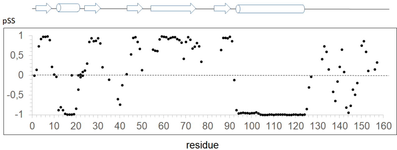
Fig. 2. The secondary structure propensities pSS of the P1 protein derived from TALOS-N on the basis of the chemical shifts of H\alpha , ^{15}N , C\alpha , C\beta and C' atoms (Shen and Bax, 2013). Positive and negative values stand for \beta -sheet and \alpha -helice predictions respectively. The predicted secondary structures are schematized above.
