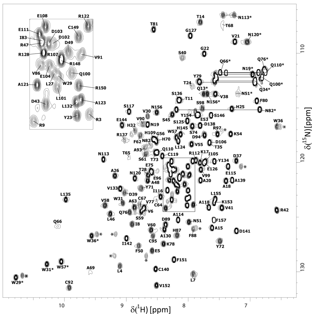
Fig. 1: 2D ^1\text{H} - ^{15}\text{N} HSQC spectrum of 200 \mu\text{M} sample of ^{15}\text{N} -labeled P1 in 100 mM NaCl, 60 mM \text{Na}_2\text{SO}_4 , 50 mM Tris buffer, pH 8 at 300K. Each backbone amide resonance is labeled with the amino acid type (one-letter code) and the number in the sequence. He1-Ne1 amino groups from tryptophanes are labeled with an asterisk (*). Also labelled with an asterisk are the assigned amide groups from glutamine and asparagine side chains, which are in addition outlined with horizontal lines.
