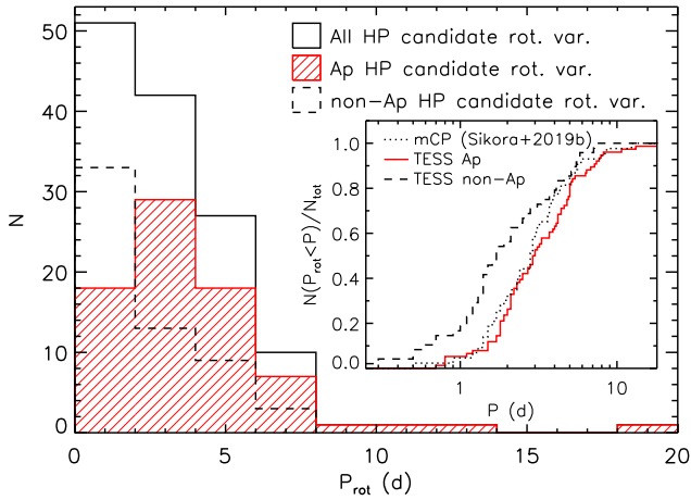
Figure 4. Distributions of the rotation periods ( P_{\text{rot}} ) obtained from the TESS light curves associated with the high-probability (HP) rotational variable candidates for the total sample (solid black), subsample of Ap stars (red hatched), and subsample of non-Ap stars (dashed black). Inset: The cumulative distribution functions associated with the P_{\text{rot}} values of the TESS stars not classified as being Ap (dashed black), the TESS stars classified as Ap (solid red), and the confirmed mCP stars having P_{\text{rot}} < 15 d (90 per cent of the sample of mCP stars) included in the survey carried out by Sikora et al. (2019a) (dotted black).
