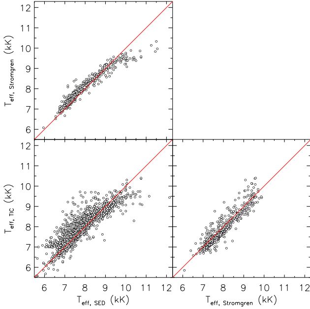
Figure 8. Comparisons between T_{\text{eff}} values derived using three methods: T_{\text{eff, TIC}} are obtained from the TESS Input Catalogue, T_{\text{eff, Stromgren}} are derived from a Strömgren colour- T_{\text{eff}} calibration, and T_{\text{eff, SED}} are derived by fitting synthetic SEDs to various photometric measurements, depending on their availability.
