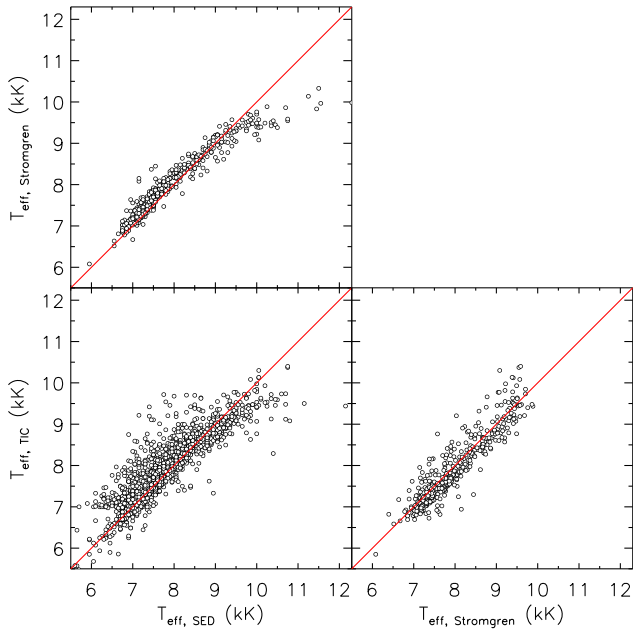
Figure 8. Comparisons between T_{\text{eff}} values derived using three methods: T_{\text{eff, TIC}} are obtained from the TESS Input Catalogue, T_{\text{eff, Strömgren}} are derived from a Strömgren colour- T_{\text{eff}} calibration, and T_{\text{eff, SED}} are derived by fitting synthetic SEDs to various photometric measurements, depending on their availability.
