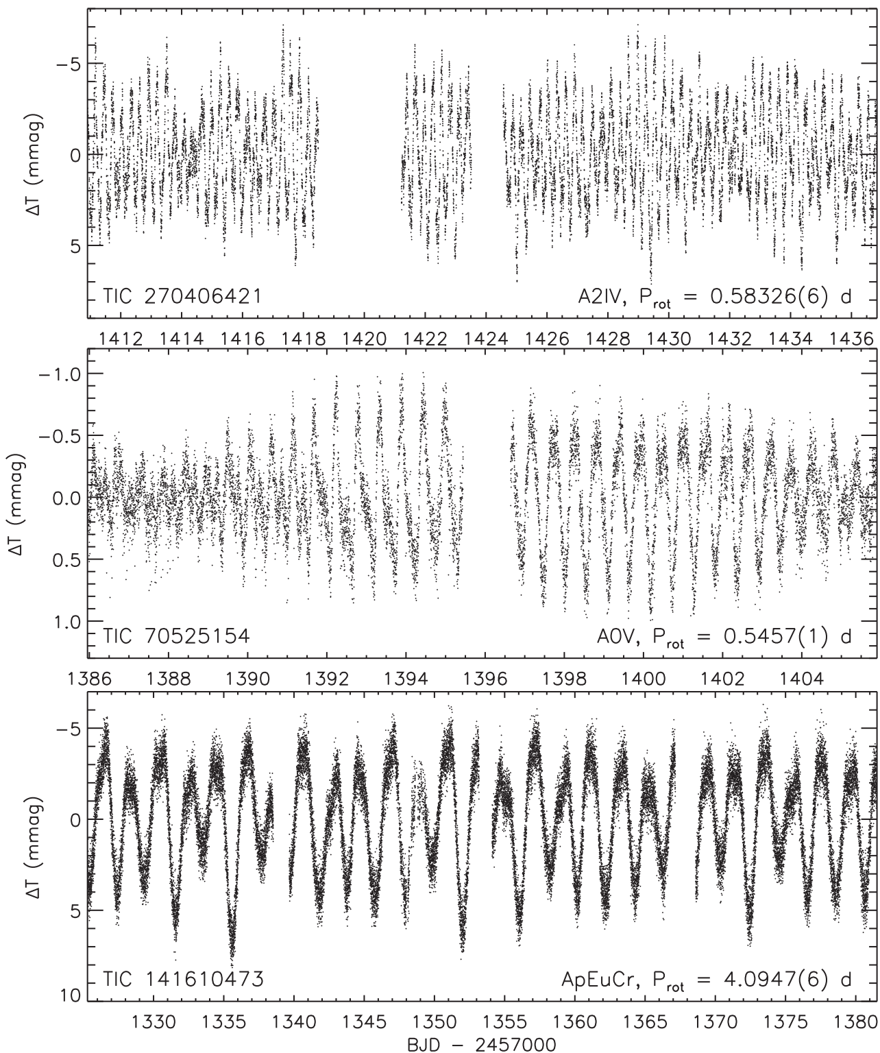
Figure 6. Examples of TESS light curves exhibiting rotational modulation with variable amplitudes (amplitude modulation, AMod).
