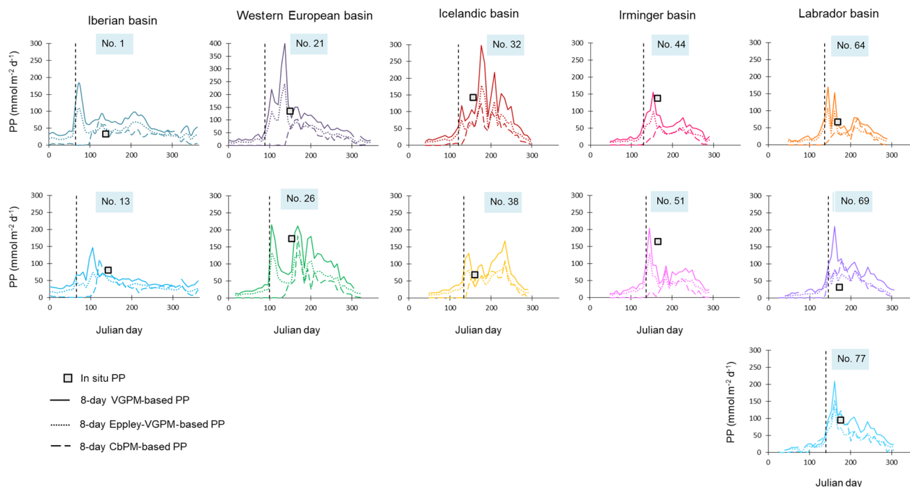
Figure 4. In situ (squares) and satellite VGPM-derived (continuous lines), VGPM-Eppley-derived (dotted lines) and CbPM-derived (dashed lines) primary production (PP; in \text{mmol m}^{-2} \text{d}^{-1} ) data at the time of our sampling and throughout the year 2014. The start of the bloom, defined by a PP increase of 30 % above the winter value, is indicated with the black vertical dashed line.
