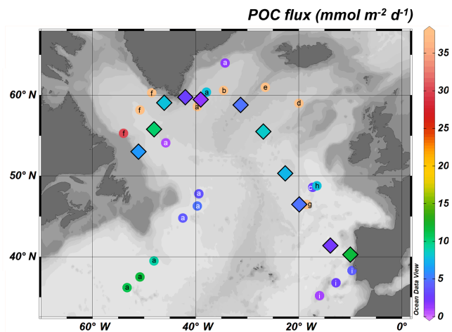
Figure 7. Comparison of the POC export fluxes from this study (diamonds with black borders) with other ^{234}\text{Th} -derived estimates of POC exports in the North Atlantic (a – Puigcorb e et al., 2017; b – Ceballos-Romero et al., 2016; c – Thomalla et al., 2008; d – Sanders et al., 2010; e – Martin et al., 2011; f – Moran et al., 2003; g – Buesseler et al., 1992; h – Le Moigne et al., 2013a; i – Owens et al., 2014).
