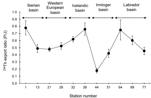
Figure 6. Variability of the ^{234}\text{Th} export ratio (i.e., the ratio of the ^{234}\text{Th} export flux over the ^{234}\text{Th} scavenged flux; P/J ratio) along the GEOVIDE section.
