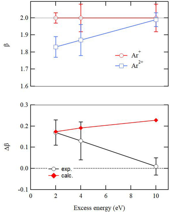
FIG. 4. Top: measured \beta values for photoelectrons in coincidence with \text{Ar}^+ and \text{Ar}^{2+} at 2, 4, and 10 eV of excess photon energy. Bottom: experimental and calculated values for \Delta\beta , the deviation of \beta from 2, as a function of excess energy.
