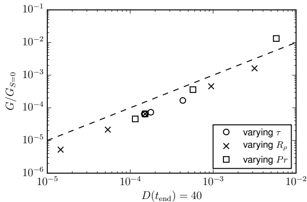
FIGURE 6. Actual damping G(S)/G_{S=0} for S = 0.1 as a function of predicted damping (4.13) from assuming locally exponential growth as m(t) = m_0 - Skt changes over time. The correct trend is recovered for all parameter combinations, although the predictions are a factor of 2-3 too small. Values of \tau are 10, 30, 100, 300 and 1000. Values of R_\rho are 1.6, 1.8, 2, 2.5 and 3. Values of Pr are 0.2, 1, 7 and 50.
