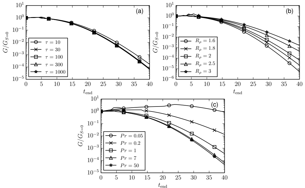
FIGURE 4. Ratio of sheared optimal gain with S = 0.1 to unsheared optimal gain for the fingering instability. Unless noted otherwise in the legend, the parameter values are Pr = 7 , \tau = 100 , R_\rho = 2 and V_p = 0 .
