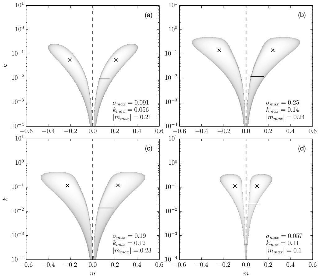
FIGURE 11. Linear stability growth rate vs. horizontal wavenumber k and vertical wavenumber m in the absence of shear, for parameters (a) base case of Pr = 7 , \tau = 1 , R_\rho = 2 and V_p = 1 , (b) increased V_p = 2 , (c) decreased R_\rho = 1.5 and (d) decreased Pr = 0.05 . Shading is logarithmic. The maximum growth rates are marked with an X. The horizontal black lines represent the paths of the non-modal optimal growth when S = 0.1 and t_{\text{end}} = 100 (a-c), and t_{\text{end}} = 60 (d), as m = m_0 - Skt .
