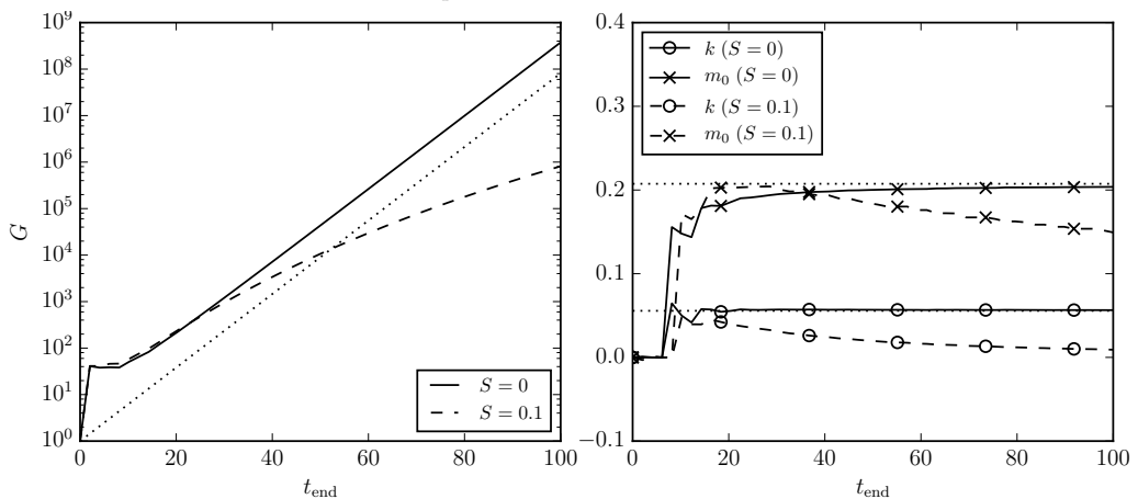
FIGURE 8. Optimized gain G and corresponding k and m_0 as a function of time interval [0, t_{\text{end}}] for the settling instability. The other parameters are Pr = 7 , \tau = 1 , R_\rho = 2 and V_p = 1 . The dotted lines indicate linear stability results for maximum growth rate and corresponding (k, m) , in the absence of shear.
