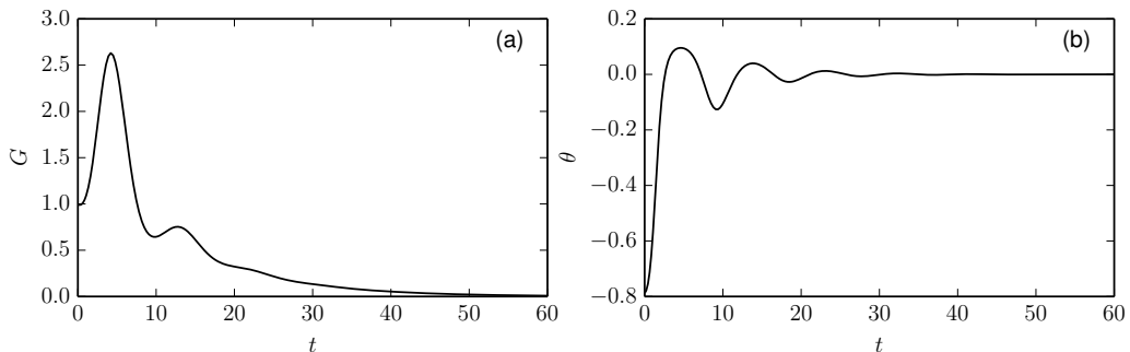
FIGURE 10. (a) Gain, as defined in (3.1), and (b) phase angle between temperature and particle perturbations as functions of time for Pr = 7 , \tau = 1 , R_\rho = 2 , V_p = 0 and initial \theta = -\pi/4 . There is initial, transient growth that decays as the phase angle decays without any sustained driving force to maintain it.
