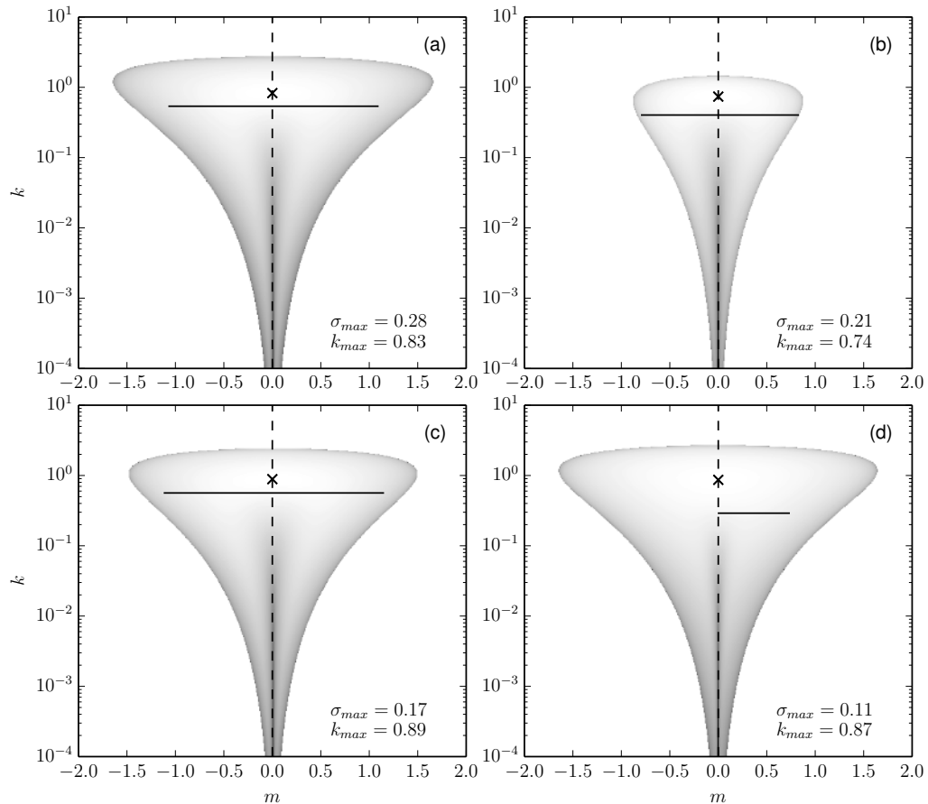
FIGURE 5. The unsheared case S = 0 : linear stability analysis growth rate vs. horizontal wavenumber k and vertical wavenumber m for the parameter combinations: (a) base case of Pr = 7 , \tau = 100 , R_\rho = 2 and V_p = 0 , (b) decreased \tau = 10 , (c) increased R_\rho = 3 , and (d) decreased Pr = 0.05 . The shading is logarithmic, and the maximum growth rates are marked with an X. The horizontal black lines represent the paths of the non-modal optimal growth from t = 0 to t_{\text{end}} for S = 0.1 according to m = m_0 - Sk t . (a-c): t_{\text{end}} = 40 , (d) and t_{\text{end}} = 25 .
