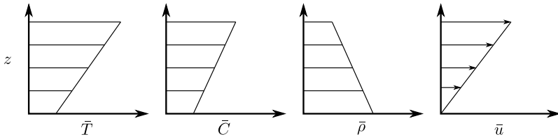
FIGURE 1. Background temperature \bar{T} , particle concentration \bar{C} , density \bar{\rho} and x -velocity \bar{u} . Within the stable overall density stratification, the particle concentration is unstably stratified.
