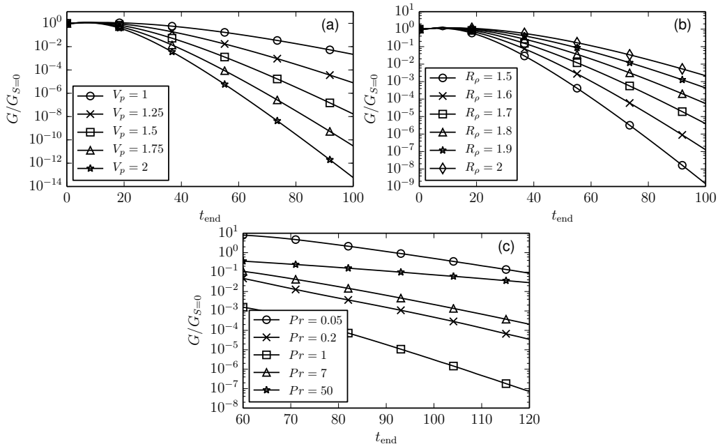
FIGURE 9. Ratio of sheared optimal gain with S = 0.1 to unsheared optimal gain for the settling instability with \tau = 1 . Other parameters are (a) Pr = 7 , R_\rho = 2 , (b) Pr = 7 , V_p = 1 , (c) R_\rho = 2 , V_p = 1 .
