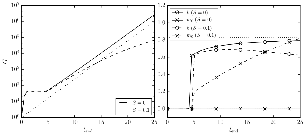
FIGURE 2. Optimized gain G and corresponding k and m_0 as a function of the time interval [0, t_{\text{end}}] for the fingering instability. The other parameters are Pr = 7 , \tau = 100 , R_\rho = 2 and V_p = 0 . The dotted lines correspond to linear stability results for the maximum growth rate and corresponding k -value, in the absence of shear.
