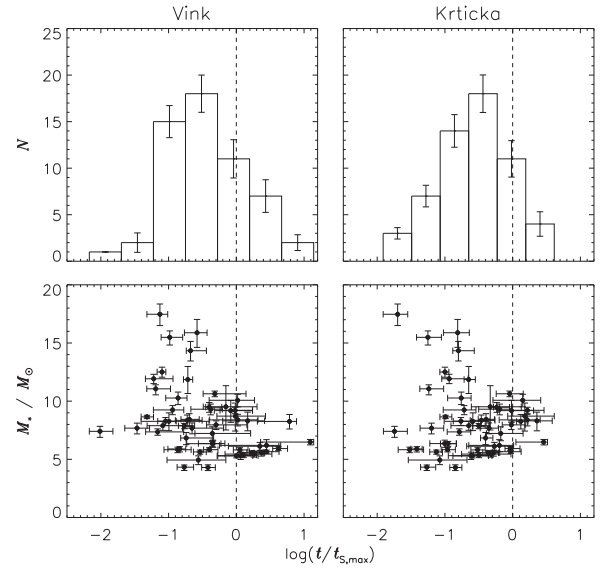
Figure 11. Top: histograms of the logarithmic ratio of age to t_{\text{S,max}} for Vink (left) and Krtička (right) mass-loss rates. Bottom: \log(t/t_{\text{S,max}}) as a function of stellar mass.
