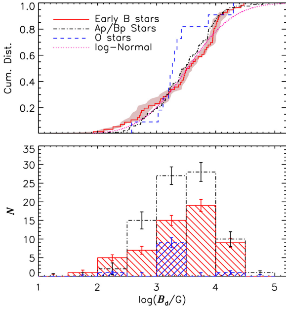
Figure 6. Cumulative distributions (top) and histograms (bottom) of the dipole magnetic field strengths B_d for early B-type stars, Ap/Bp stars, and magnetic O-type stars. The grey shaded region in the top panel indicates the 1\sigma uncertainty.
