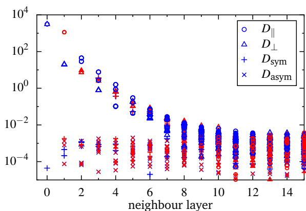
Fig. 4 Effective interactions in a hexagonal hard-disk crystal with L = 32 . Larger blue symbols are positive values, smaller red symbols are negative values. K = 2N \times 3.5 \times 10^6 recordings, obtained from 336 independent trajectories. Surface fraction \phi = 0.85 . These data required around 300 000 CPU core hours.
