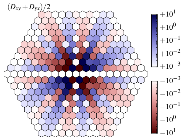
Fig. 6 Some linear combinations of matrix elements D_{\alpha\beta}(\mathbf{n}) for several \mathbf{R}_n . The antisymmetric off-diagonal (D_{xy} - D_{yx})/2 vanishes to within statistical noise.
