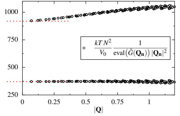
Fig. 7 Dispersion curves used to obtain the elastic moduli in the limit |\mathbf{Q}| \rightarrow 0 , here for L = 100 . The dotted lines indicate values from a different numerical method working at |\mathbf{Q}| = 0 .
