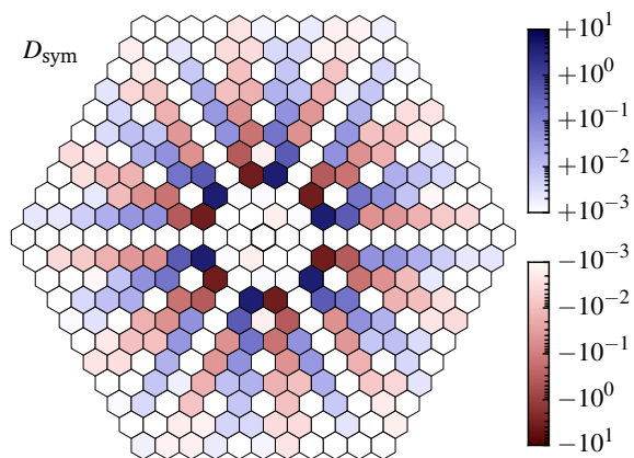
Fig. 5 Matrix elements of D(\mathbf{n}) in rotated frames of reference, for several \mathbf{R}_n . The center of the hexagon corresponds to \mathbf{R}_n = \mathbf{0} . The antisymmetric off-diagonal D_{\text{asym}} vanishes to within statistical noise. The reflection anti-symmetry of D_{\text{sym}} imposes that the elements of D_{\text{sym}} are zero for the first two neighbour layers. All elements of D_{\text{sym}} are small compared to D_{\parallel} and D_{\perp} .
