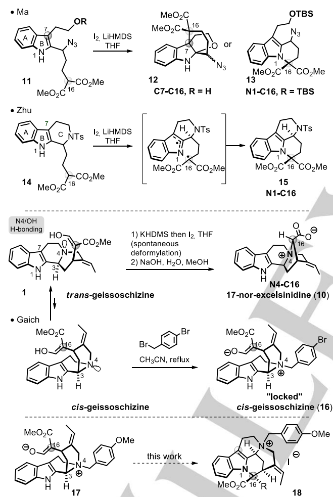
Scheme 2. Divergent oxidative couplings for the formation of the N1-C16 or C7-C16 bonds and conformational studies of geissoschizine. 16-17 zwitterions
