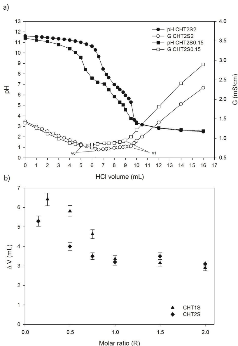
377 378 Figure 5. a) plots of simultaneous titration of CHT2S samples ( R=0.15 and R=2 ) dissolved in NaOH 0.01M followed by pH-metry and 379 conductometry; b) Evolution of the difference between the equivalent volumes ( \Delta V = V_1 - V_0 in mL) measured from conductometric titrations 380 of CHT1S and CHT2S series prepared from 0.15 < R < 2 . Decreasing \Delta V values reveals a decrease of free glucosamine groups and an 381 increase of DS.
