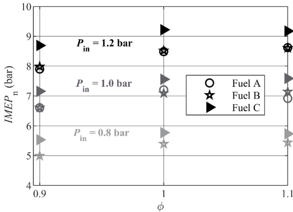
Figure 4. Net Indicated Mean Effective Pressure for the various fuels and intake pressures.
