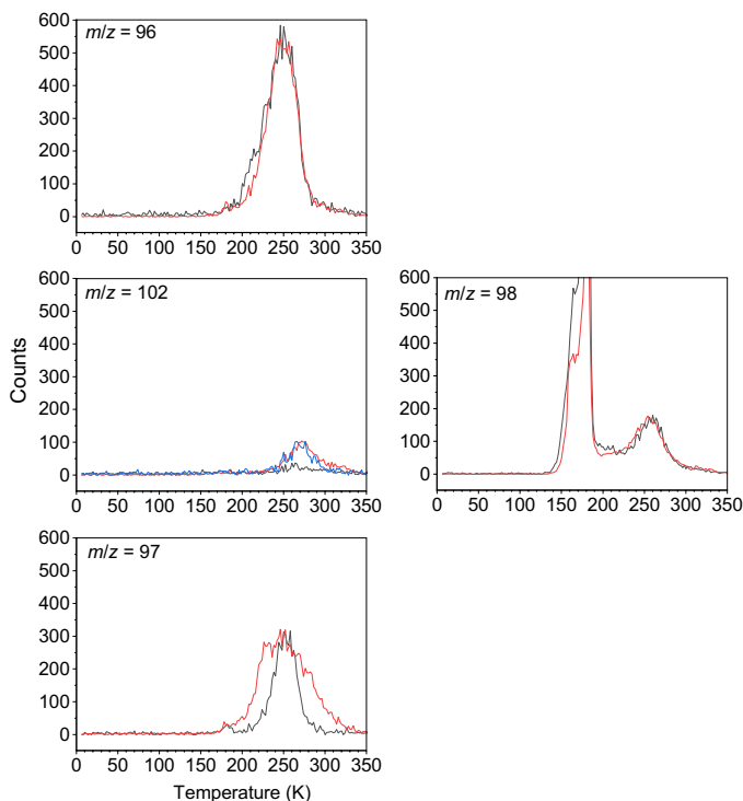
Fig. 3. TPD profiles of photoionized \text{H}_5\text{CPO}_3 isomers along with their ^{18}\text{O} and ^{13}\text{C} substituted counterparts ( \text{H}_5\text{CP}^{18}\text{O}_3 and \text{H}_5^{13}\text{CPO}_3 ) recorded at m/z = 96 , 102, and 97 subliming from the processed \text{PH}_3 + \text{H}_2\text{O} + \text{CH}_4 (top), \text{PH}_3 + \text{H}_2^{18}\text{O} + \text{CH}_4 (center), and \text{PH}_3 + \text{H}_2\text{O} + ^{13}\text{CH}_4 (bottom) ices. The TPD profiles are shown for photon energies of 9.93 eV (black), 10.35 eV (blue), and 10.49 eV (red). The middle right graph shows m/z = 98 for the \text{PH}_3 + \text{H}_2^{18}\text{O} + \text{CH}_4 systems to demonstrate the presence of the \text{H}_6\text{CP}_2\text{O} compounds, which would also be present in the m/z = 96 ( \text{PH}_3 + \text{H}_2\text{O} + \text{CH}_4 ) and m/z = 97 ( \text{PH}_3 + \text{H}_2\text{O} + ^{13}\text{CH}_4 ) signals.
