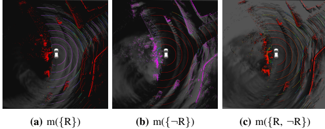
Fig. 5: Model-free evidential road grid mapping. The accumulated evidential grid is overlaid with the point-level evidential mass values generated from the LIDAR sensor
