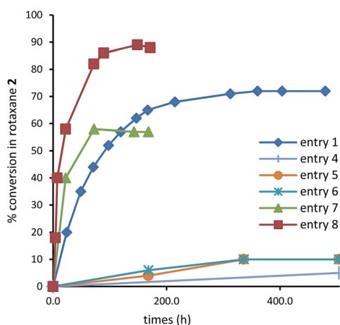
Fig. 1 Kinetics comparison of the slippage-on relative to the formation of rotaxane 2 from 1. Corresponding experimental procedures are given in Table 1. Conversion ratio of rotaxane 2 was calculated from subsequent 1 H NMR analysis of the mixture. For sake of clarity, curves corresponding to entries 2 and 3 were omitted.
