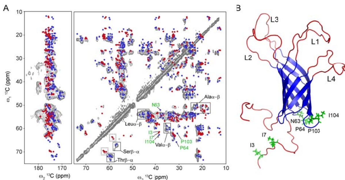
Supplementary Fig. 1. (A) Two-dimensional ^{13}\text{C} - ^{13}\text{C} PDSD correlation spectrum of the membrane-embedded KpOmpA TM domain reconstituted in E. coli PLE vesicles (PLR=0.5, w/w) recorded with a PDSD mixing time of 40 ms at a MAS frequency of 12 kHz and at 20°C (sample temperature). Expected intraresidue C-C correlations predicted from solution NMR chemical shifts of KpOmpA TM domain (BMRB accession code: 15651) after correction for isotope effect (squares). (B) Cartoon representation of the solution NMR structure of KpOmpA TM domain (PDB accession code: 2K0L). Color-coding in (A) and (B): red, extracellular loops (L1 to L4), N- and C-term extremities; blue, transmembrane \beta -sheets ( \beta 1 to \beta 8) and periplasmic turns (T1 to T3). Residues with backbone \text{C}^\alpha/\text{C}^\beta correlations that could not be observed at similar peak position than those predicted by solution NMR chemical shifts are labeled in green.
