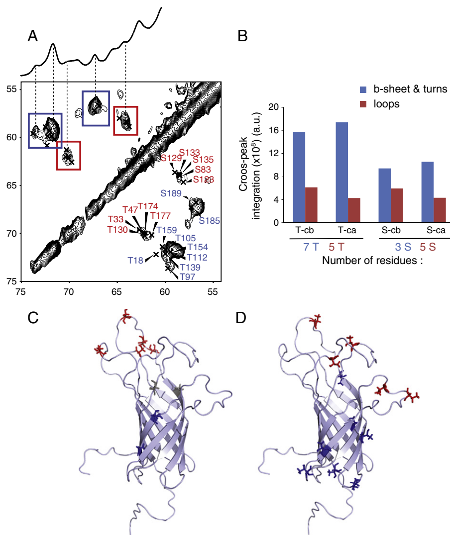
Fig. 3. (A) Selected region of the 2D ^{13}\text{C} , ^{13}\text{C} PDSO correlation spectrum showing backbone \text{C}^\beta - \text{C}^\alpha correlations of the Thr and Ser residues of KpOmpA TM domain. Solution NMR assignments are indicated when available. Open rectangles represent spectral regions used for signal integration, expected correlations were obtained from available solution NMR chemical shifts of KpOmpA TM domain (BMRB 15651 [9]) after correction due to ^2\text{H} isotope effect. (B) Integrations of spectral regions corresponding to Thr and Ser residues within random-coil (red bars) and \beta -sheet-like (blue bars) protein segments plotted onto the number of residues. (C) Distribution of Ser residues within KpOmpA TM domain (PDB ID: 2KOL). (D) Distribution of Thr residues within KpOmpA TM domain. For (C) and (D) the color code is: residues within \beta -sheet TM and turns segments are in blue, those within the extracellular loops are in red. Two unassigned residues are labeled in dark gray. (For interpretation of the references to color in this figure legend, the reader is referred to the web version of the article.)
