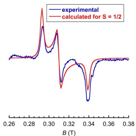
Figure S5. EPR spectra of the two-reduced species (blue) ((microwave power = 1 mW, modulation amplitude = 8 Gauss, gain = 50 db, temperature = 30 K) and simulation (red) considering S = 1/2 with the following g_{\text{eff}} values g_{\text{xeff}} = 2.3499 , g_{\text{yeff}} = 2.2205 , g_{\text{zef}} = 2.0293
