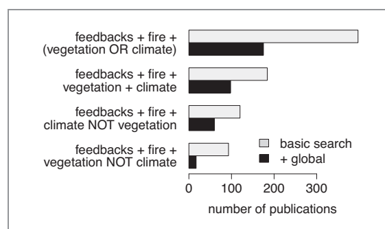
Figure 2. Summary of how fire feedbacks in the Earth system are represented in published literature on Web of Science (see SI for methods available at stacks.iop.org/ERL/13/033003/mmedia ). Only about half of the available studies about fire feedbacks consider both vegetation and climate. Global studies on feedbacks with climate are three times more likely than those with feedbacks on vegetation, although vegetation feedbacks appear to be better recognised in local/landscape-level studies.
