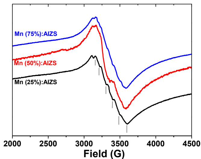
Fig. 2 EPR spectra recorded at 20 K of orange-emitting AIZS loaded with 25, 50 and 75% \text{Mn}^{2+} .
