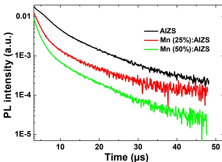
Fig. 8 PL lifetimes of orange-emitting AIZS and of the corresponding Mn:AIZS QDs at the PL maximum wavelength.
