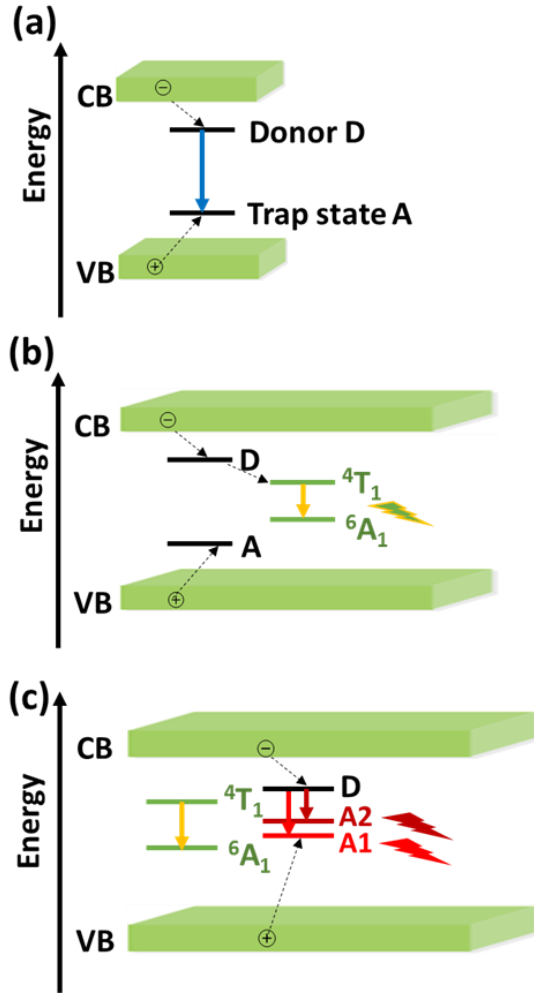
Fig. 7 Schematic illustration of the PL mechanism of (a) AIZS and (b-c) Mn:AIZS QDs. The solid arrows correspond to radiative relations while the dotted arrows show the non-radiative relaxations.
