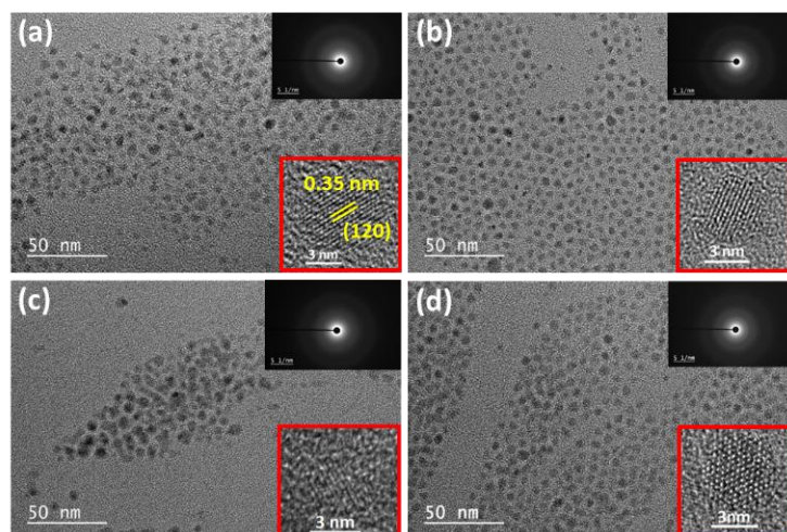
Fig. 3 TEM and HR-TEM images of (a) orange-emitting AIZS and (b-d) Mn:AIZS QDs loaded with 25, 50 and 75% Mn 2+ , respectively. The insets show SAED patterns.
