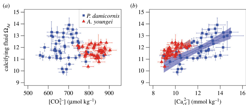
Figure 4. Relative influences on coral calcifying fluid \Omega_{Ar} . Sensitivity of \Omega_{Ar} to (a) [\text{CO}_3^{2-}]_{cf} and (b) [\text{Ca}^{2+}]_{cf} . Colours are the same as in figure 2.
