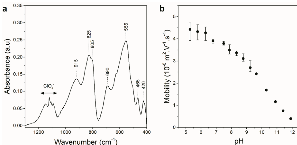
Figure 3. (a) Infrared spectrum obtained on a powder of DW_0 . (b) Evolution of the electrophoretic mobility as a function of the pH on a dilute suspension of DW_0 .
