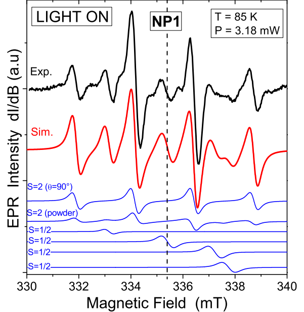
Figure 9: (color online) Simulated (red) and experimental (black) EPR spectra recorded on NP1 at 85 K in saturated conditions ( P = 3.18 mW) under illumination. Various contributions to the simulation are display (blue), all divided by a factor 3.
