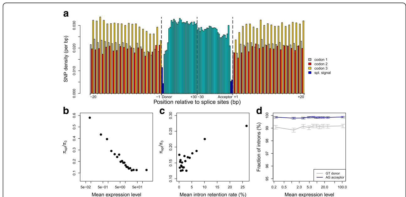
Fig. 6 Variation in selective constraints on splice signals in human genes. a SNP density was measured in the vicinity of exon-intron boundaries (first and last 30 bp of introns and 20 bp of flanking exons), over all introns located between coding exons ( n = 170,015 ). Splice sites (first and last 2 bp of introns) are displayed in dark blue , other intron positions in light blue . Within coding regions, the SNP density at each site was computed separately for the three codon positions ( gray : position 1, red : position 2, yellow : position 3). b The level of selective constraints on splice signals increases with gene expression level. Introns were classified into bins of equal sample size, according to gene expression levels. Within each bin, the fitness impact of mutations on splice sites was estimated by measuring the ratio \pi_{spl}/\pi_3 , where \pi_{spl} is the SNP density at splice sites and \pi_3 is the SNP density at flanking third codon positions. c The level of selective constraints on splice signals decreases with increasing IR rate. Introns were classified into bins of equal sample size according to their average retention rate and the ratio \pi_{spl}/\pi_3 was measured in each bin. d The fraction of introns with consensus splice signals does not vary with gene expression level. The proportion of introns matching the consensus splice donor (GT) and the proportion of introns matching the consensus splice acceptor (AG) was computed for each bin of expression level. Error bars represent the 95% CI of this proportion. b, d Mean expression levels (RPKM) are represented in log scale
