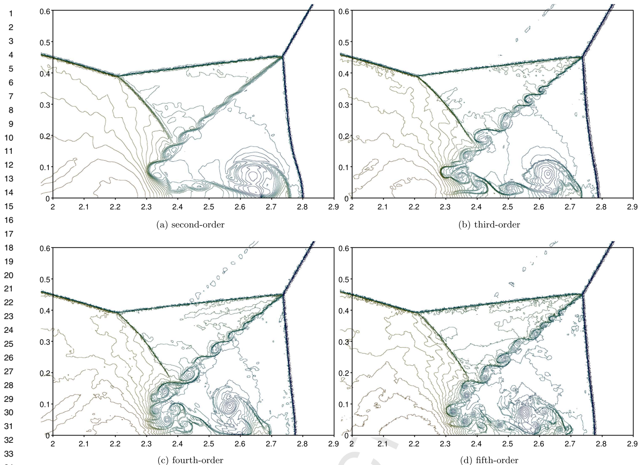
Fig. 30. High-order DG with proposed WENO and positivity preserving with irregular triangular elements ( h = 1/200 ) in (x, y) \in [0, 4] \times [0, 1] . Shown are zoom-in views around the Mach stems at t = 0.2 with 41 equidistance density contour lines from 1.5 to 22.5.
