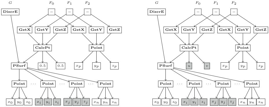
Fig. 8 Black DAGs representing the optimization problems to be solved, when (u, v) is constant (left) and variable (right) [32]
