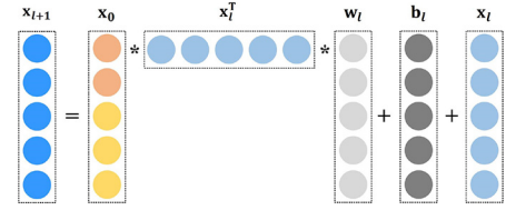
Fig. 4. Bite-wise interactions.
