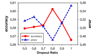
Fig. 10. Impact of different dropout ratio.
