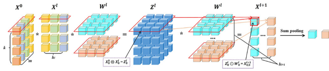
Fig. 5. Vector-wise interactions.
