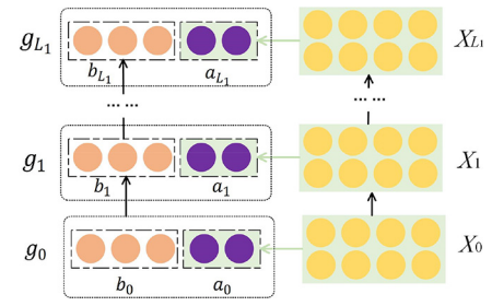
Fig. 6. Hybrid interactions.
