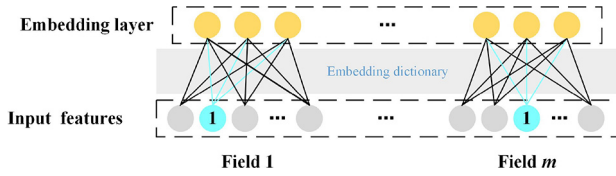
Fig. 2. Filed embedding.
