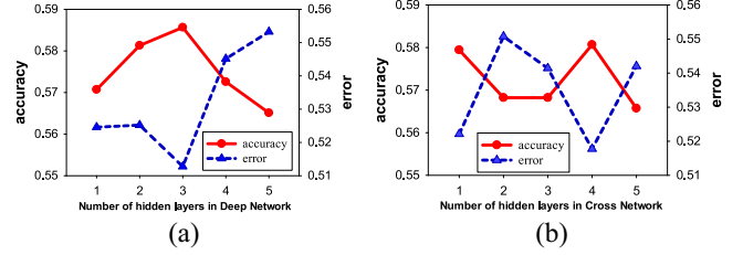
Fig. 8. Impact of number of hidden layers in the deep network and the CrossNet. (a) Deep network. (b) Cross network.
