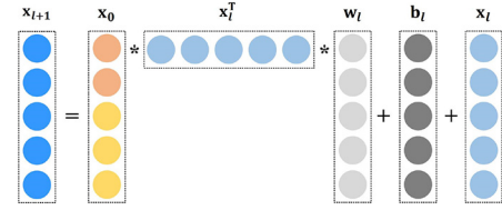
Fig. 4. Bite-wise interactions.
