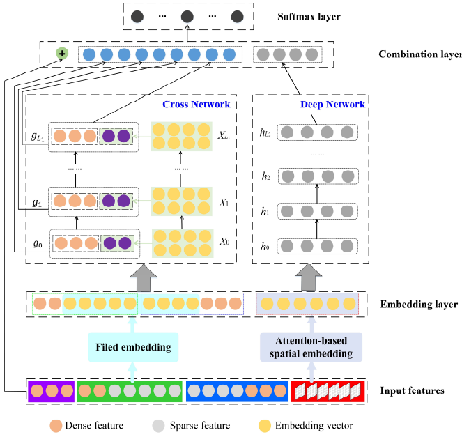
Fig. 1. DeepStore framework.
