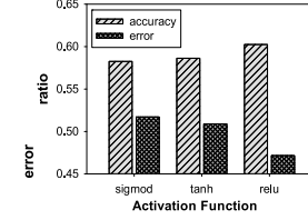
Fig. 11. Impact of different activation function.
