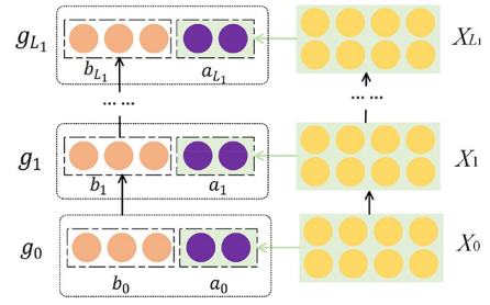
Fig. 6. Hybrid interactions.
