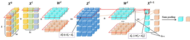
Fig. 5. Vector-wise interactions.
