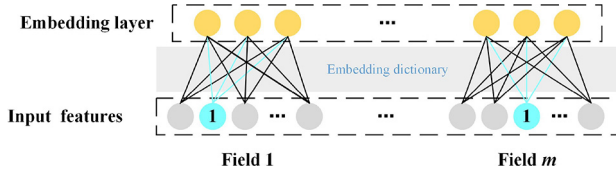
Fig. 2. Field embedding.
