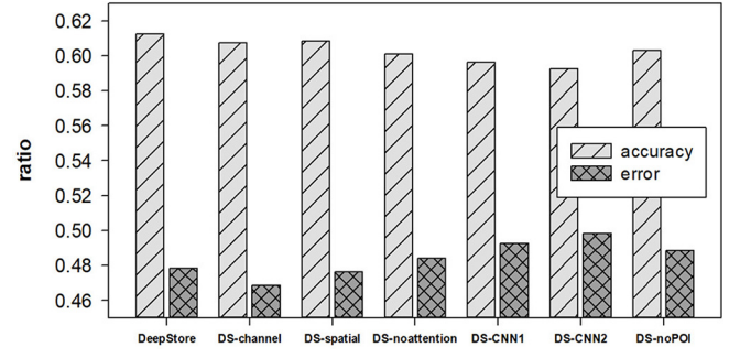
Fig. 7. Performance comparison of DeepStore and its variants.
