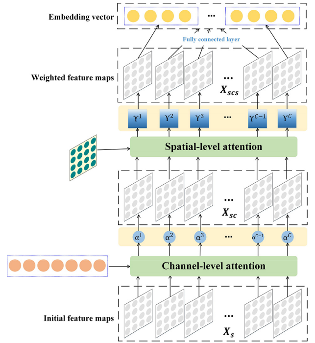
Fig. 3. Attention-based spatial embedding.
