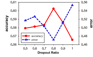
Fig. 10. Impact of different dropout ratio.
