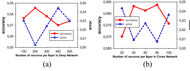
Fig. 9. Impact of number of neurons per layer in the deep network and the CrossNet. (a) Deep network. (b) Cross network.
