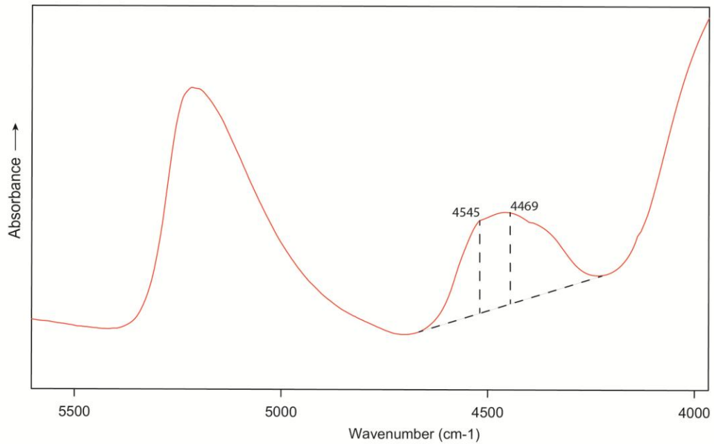
Figure 4: Example of spectrum obtained by IR spectroscopy presenting two combination bands. A first band around 5\ 220\text{cm}^{-1} produced by molecular water and a second produced by Si-OH groups at around 4,300\text{-}4,600\ \text{cm}^{-1} . The hydration ratio is calculated by measuring the components at 4,545\text{cm}^{-1} and 4,469\text{cm}^{-1} . [1 -column]
