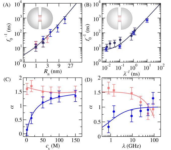
Figure 4: (A) Inverse of the low frequency cut-off f_0 as function of the nanopore radius R_n , for a charged nanopore with surface charge \Sigma = 60 \text{ mC/m}^2 , salt concentration c_s = 20 \text{ mM} , and desorption frequency \lambda = 100 \text{ GHz} (full symbols). We also report results obtained with a neutral nanopore (open symbols), and using Brownian simulations (stars). The solid line is the prediction in Eq. (10) with k = 22 \text{ m/s} . (B) Inverse of the low frequency cut-off f_0 as a function of the inverse desorption frequency \lambda^{-1} for a nanopore with radius R_n = 1 \text{ nm} . (C) Slope \alpha of the PSD of the number of free particle (blue disks) and number of bounded particle (red squares), for a charged nanopore with surface charge \Sigma = 60 \text{ mC/m}^2 , desorption frequency \lambda = 0.8 \text{ GHz} , and nanopore radius R_n = 2 \text{ nm} . Lines are guides to the eye. (D) Slope \alpha as a function of the desorption frequency for a charged nanopore with surface charge \Sigma = 60 \text{ mC/m}^2 , nanopore radius R_n = 1 \text{ nm} , and salt concentration c_s = 20 \text{ mM} . Lines are guides to the eye.
