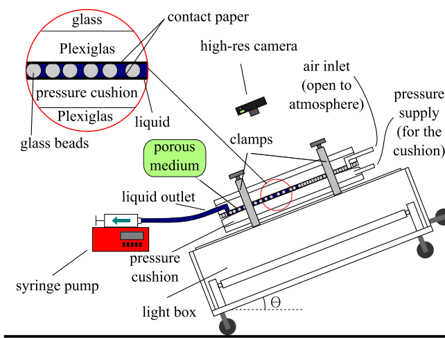
FIG. 1. Diagram of the experimental setup showing the cell with the porous medium made of a single layer of glass beads. The camera, light box, and cell are all connected to a common frame that can be inclined by an angle \theta , as shown. The liquid outlet on the left is connected to a syringe pump that withdraws the liquid. The water inlet for the cushion (on the right) is connected to a bottle which is kept at a high level ( \approx 3 m). This is to keep the cushion pressurized. There is no connection between the water in this cushion and the fluids in the porous medium.
