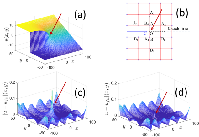
FIG. 2. Spatial distribution of voltage field and effect of crack tip mispositioning. (a) Map of voltage field, u(x, y) in a 200 \times 100 square lattice under TS loading. The crack lies along x in the middle of the strip, so that the next bond about to break is at the map center (red arrow) and the external applied voltage difference, 2U_{ext} , is at the value required to break this bond. Equations 3 and 4 are expected to describe this field. (b) Zoom on the tip vicinity emphasizing the lattice discreteness. The difficulty is to place the continuum-scale crack tip in this discrete lattice. At first, this tip is placed in the middle, \mathbf{O} , of the bond to break. (c) Absolute difference |u_{fit} - u|(x, y) between the voltage field of panel (a) and the one, u_{fit}(x, y) , fitted using Eqs. 3 and 4, with 1 \leq n \leq 11 (6 terms). The fit is very good everywhere, except in the very vicinity of the crack tip (red arrow). (d) Absolute difference |u_{fit} - u|(x, y) after correcting for the mispositioning and placing the continuum-scale tip at the proper position, \mathbf{C} , using the iterative procedure depicted in the text. The fit is now very good everywhere.
