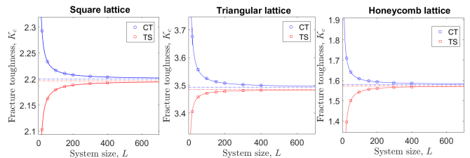
FIG. 3. Fracture toughness K_c plotted as a function of the system size L , in both TS and CT loading configurations, for the three lattice geometries: square, honeycomb and triangular. K_c is obtained by fitting the voltage field u(x, y) using Eqs. 3 and 4 after having corrected the tip mispositioning using the iterative procedure depicted in the main text. For all curves, the continuous line is a power-law fit K_c = a/L^p + K_c^\infty . The material constant K_c^\infty obtained in the thermodynamic limit ( L \rightarrow \infty ) is independent of the loading conditions (dotted horizontal lines). These values are reported in the fourth line of Tab. 1.
