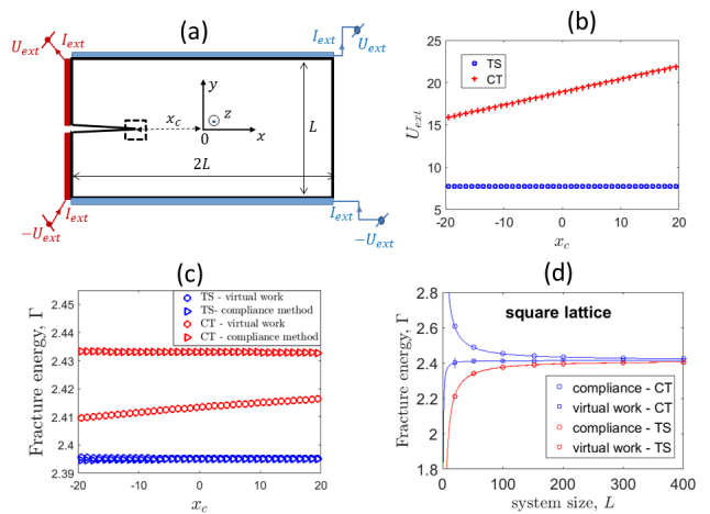
FIG. 1. (a) Sketch and notation of the simulated fuse lattice. The external voltage difference 2U_{ext} is imposed between the blue electrodes in the TS configuration, and between the red ones in the CT configuration. In response, a total current I_{ext} flows through the network. U_{ext} and I_{ext} are the analog of loading displacement and loading force in experimental mechanics. (b) U_{ext} value at breaking onset as a function of crack tip position x_c , in a 200 \times 100 square lattice. (c) \Gamma vs x_c in the same system. Note that y -axis ranges from 2.39 to 2.46. \Gamma is nearly independent of x_c , no matter how it is measured and the loading configuration. (d) Size dependency of \Gamma averaged over x_c . For small sizes, \Gamma depends on both the measurement method and loading configuration. However, the differences vanishes as L \rightarrow \infty . All curves were fitted by \Gamma = a/L^p + \Gamma_\infty , and the fitted value \Gamma_\infty is a material constant, independent of both loading configuration and measurement method. Panel (d) concerns the square geometry but the same features were observed in triangular and honeycomb lattices. Table 1 (third line) provides the values \Gamma measured in the three lattice geometries.
