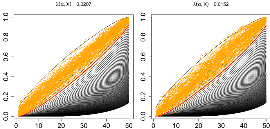
FIG 4. Illustration of the \lambda = \lambda(\alpha, X) calibration method on one realization of the data X . Black curves: beta template k \mapsto t_k(\lambda) for some range of \lambda values. Orange curves: ordered p -values (after permutation) k \mapsto p_{(k:m)}(g_j.X) for 1 \leq j \leq B = 1000 . Red curve: k \mapsto t_k(\lambda(\alpha, X)) . Left panel : full null, right panel : half of true nulls (see text). (Parameters m = 50 , \alpha = 0.2 , n_1 = 50 , n_2 = 50 , \delta = 3 .)
