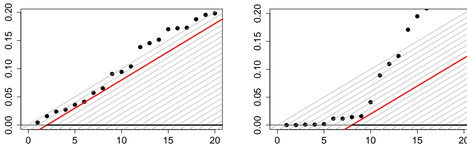
FIG 1. Illustration of the Simes post hoc bound (3) according to the expression (5), for two subsets of \mathbb{N}_m (left display/right display), both of cardinal 20 and for m = 50 . The level is \alpha = 0.5 (taken large only for illustration purposes). Black dots: sorted p -values in the respective subsets. Lines: thresholds k \in \{u + 1, \dots, |S|\} \mapsto \alpha(k - u)/m (in red for u = |S| - V(S) , in light gray otherwise). The post hoc bound V^{\text{Sim}}(S) corresponds the length of the bold line on the X -axis.
