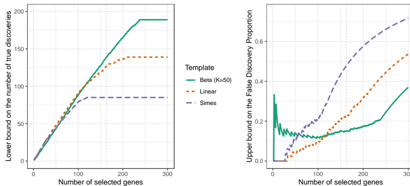
FIG 5. Confidence bounds on the number of true positives (left) and on the proportion of false positives (right) for several reference families: Simes reference family (long-dashed purple curve), linear template after \lambda -calibration (dashed red curve), and beta template after \lambda -calibration (solid green curve).
