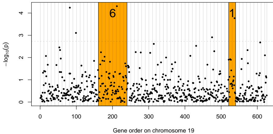
FIG 7. Evidence of locally-structured signal on chromosome 19 detected by the bound (15).
