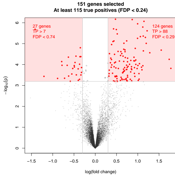
FIG 6. Post-hoc inference for volcano plots
