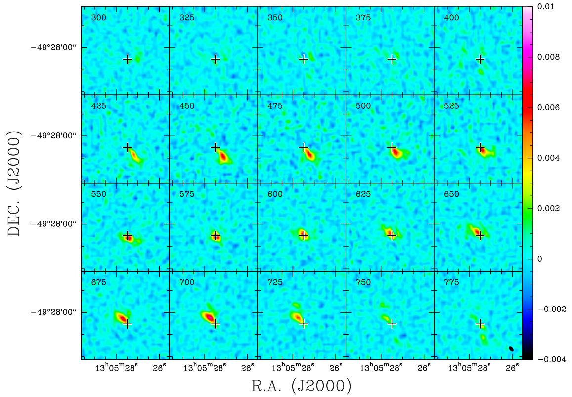
Fig. A.6. \text{CH}_3\text{C}_2\text{H} 5_0 \rightarrow 4_0 channel maps. For the units of velocity, ordinate, and wedge as well as the position of the crosses, see Fig. A.1. The value 0.01 Jy corresponds to \approx 0.42 K. The beam size is shown in the lower right corner of the figure.
