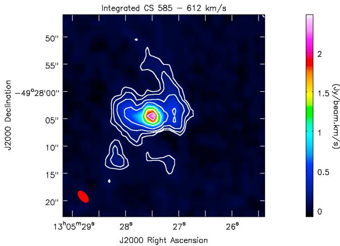
Fig. 22. Primary beam corrected CS J = 2 \rightarrow 1 emission (Briggs weighting with a robustness parameter of 0.0) integrated over the velocity interval 585–612 km s -1 , the near systemic velocity range, where nuclear absorption is not as strong as at adjacent velocities. Contours are 0.025, 0.05, 0.1, 0.2, 0.4, 0.6, and 0.8 times the integrated peak flux density of 2.48 Jy km s -1 beam -1 . Overall, line absorption plays a lesser role than in Fig. 21. While the southern region of enhanced emission is part of the southeastern arm, the hotspot around 7'' farther to the east is (as in Fig. 21) a separate feature, possibly related to Knot B of Marconi et al. (2000; see our Sect. 4.1.3).
