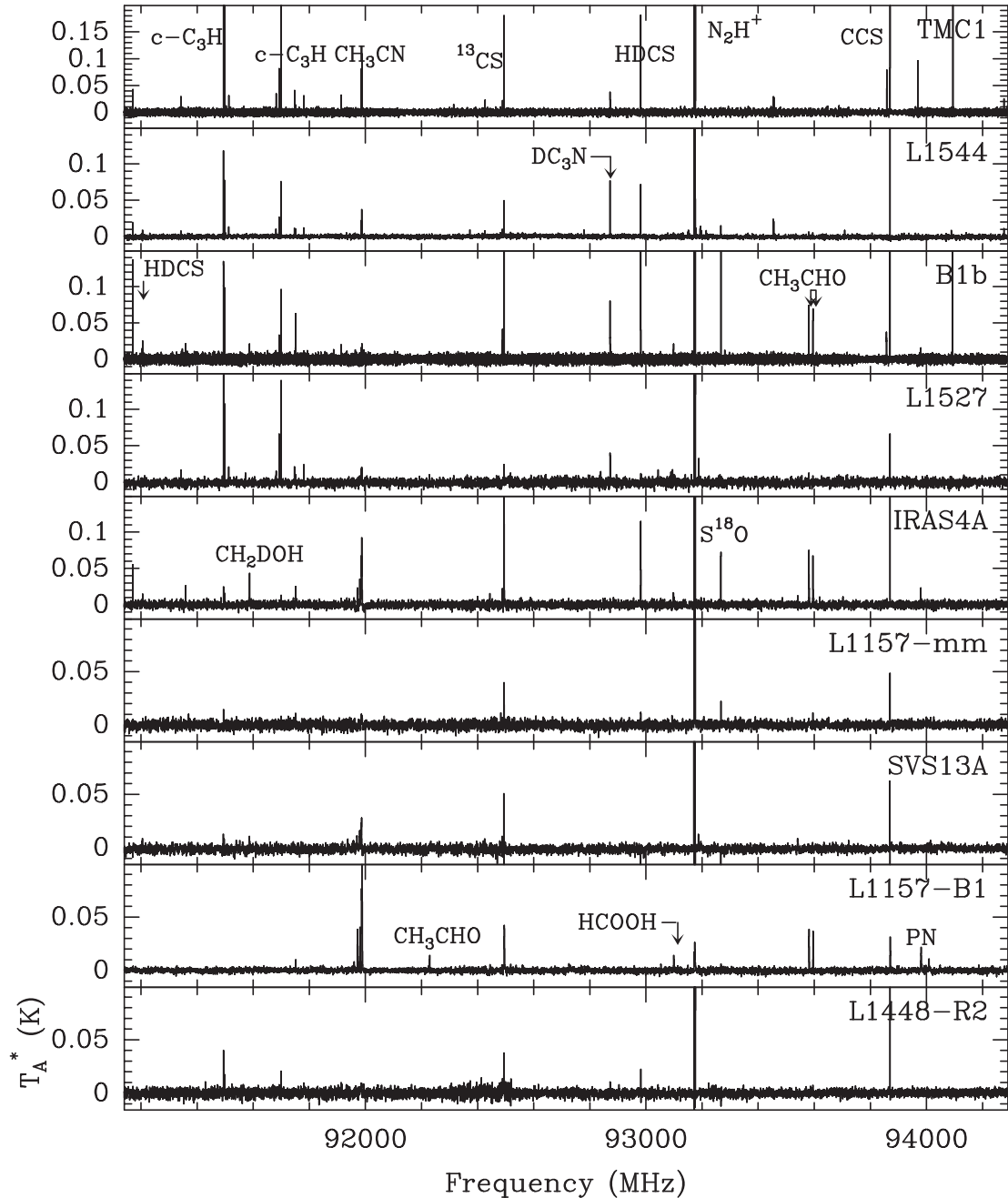
Figure 1. Molecular line emission detected with ASAI in the spectral bands: 91100–94300MHz. The spectral resolution is 350 kHz for all sources, except for TMC1 (100 kHz). The TMC1 data were taken from Marcelino et al. (2009).
