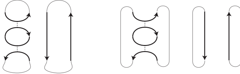
FIGURE 4. Untwisting the full twist given by two crossings that would yield a Seifert circle either reduces by two the number of crossings and the number of Seifert circles (left) or only reduces the number of crossings (right).
