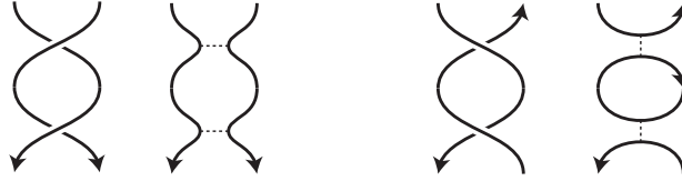
FIGURE 3. A face with two edges may (right) or may not (left) produce a Seifert circle.
