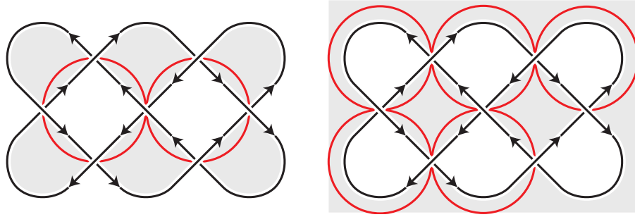
FIGURE 2. The two checkerboard surfaces associated to a positive planar link diagram and two bases of their first homology group (in red).
