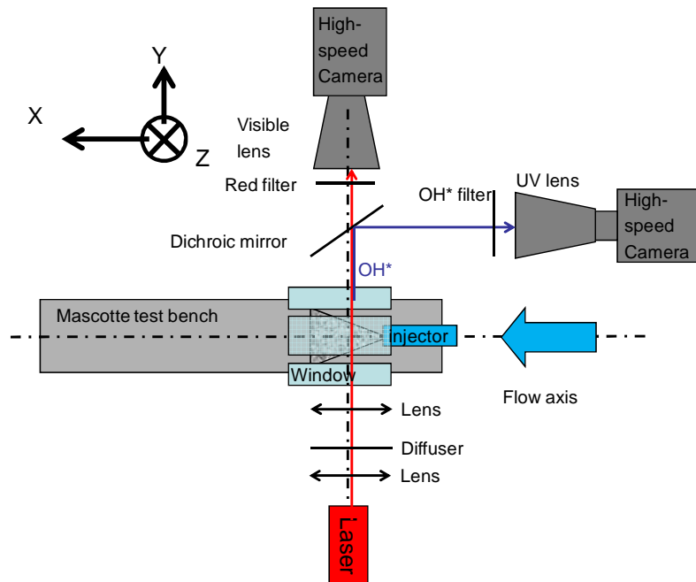
Figure 4: Imaging setup arrangement (top view) with shadowgraphy and chemiluminescence visualizations
