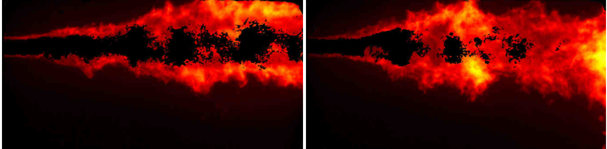
Figure 8: Superimposition of instantaneous shadowgraphs (black) and OH* emission images (colors), in cases of LOX/H2 (left) and LOX/CH4 (right)
