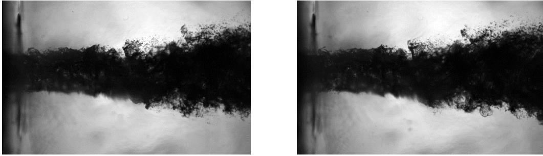
Figure 2: Instantaneous image pair of the LOX/H 2 flame, recorded at 7.5 kHz in the A-10 conditions [6]
