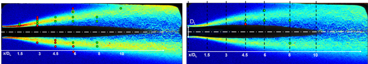
Figure 9: Superimposition of the Abel transform of OH* emission images (color), the time averaged LOX jet contour (black) and the PDI measurement locations (dots), in the cases of the LOX/H2 (left) and LOX/CH4 (right) flames.
