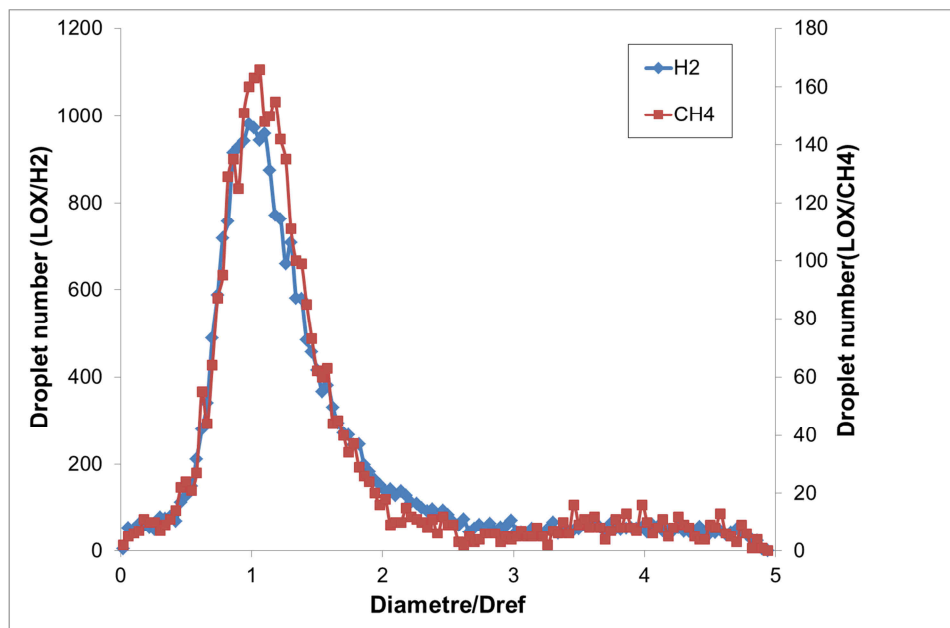
Figure 10: Example of droplet size distribution obtained with PDI at the same location, in the LOX/H 2 flame (blue) and LOX/CH 4 flame (red).
