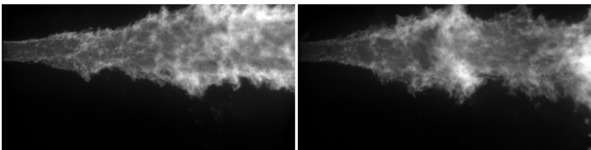
Figure 7: Instantaneous OH* images of the LOX jet flame, with hydrogen (left) and methane (right)
