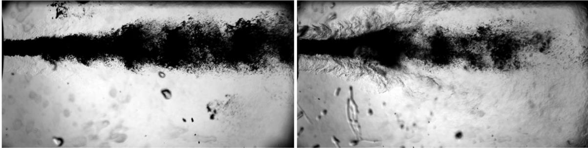
Figure 6: Instantaneous shadowgraph images of the LOX jet flame, with hydrogen (left) and methane (right)
