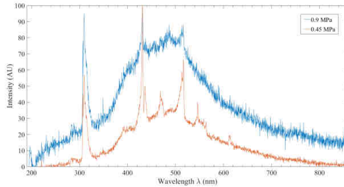
Figure 3: Emission spectra of the LOX/CH 4 flame.
