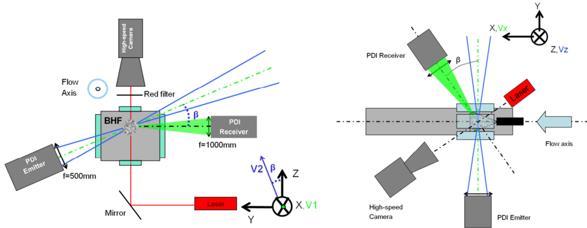
Figure 5: PDI and shadowgraphy arrangement in the vertical injection plane (left) and in the horizontal plane (right)
