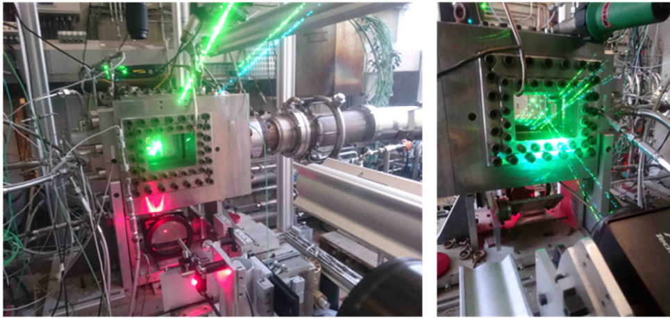
Figure 1: Illustrations of the optical setup from both sides of the MASCOTTE test bench
