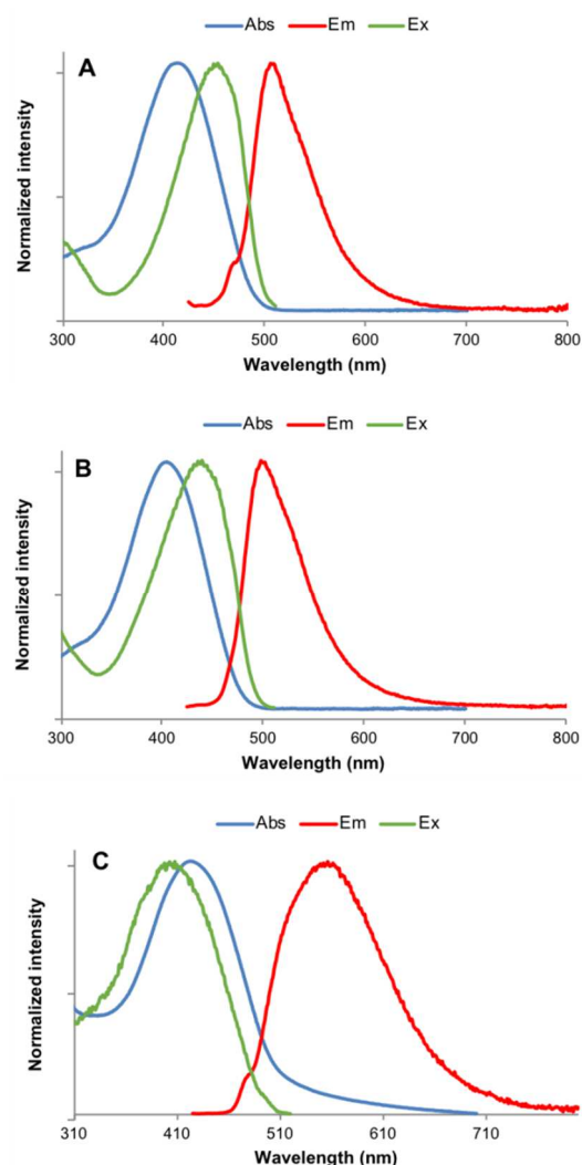
Fig. 3. Normalized absorption (blue), excitation (Em. 525 or 600 nm, slit 5 nm, green) and emission (Ex. 410 nm, slit 5 nm, red) spectra of coumarin 8 in DMSO (A), EtOH (B) and PBS (C) at 25 °C. Please note: the recorded absorption spectrum of 8 in PBS is due both to light scattering (by aggregates) and absorption.
