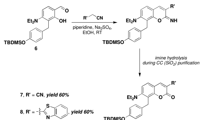
Scheme 3. Synthesis of 8-substituted 7-(diethylamino)coumarin dyes 7 and 8 (CC ( \text{SiO}_2 ) = column chromatography over silica gel).
