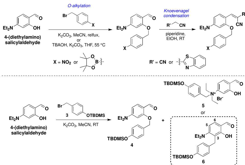
Scheme 2. (Top) Published syntheses of NTR- and peroxyxynitrite-responsive self-immolative "covalent-assembly" type probes based on O -alkylation of 4-(diethylamino)salicylaldehyde with 4-nitrobenzyl bromide or 4-(pinacolboronate)benzyl bromide and subsequent Knoevenagel condensation reaction (TBAOH = tetrabutylammonium hydroxyde) [5p],[5am]; (bottom) alkylation of 4-(diethylamino)salicylaldehyde with 4- OTBDMS benzyl bromide 3 leading to unexpected Friedel-Crafts alkylation product 6 .
