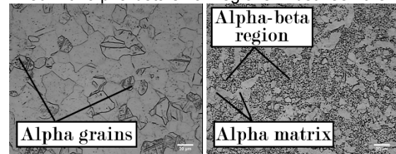
Fig. 1. Microstructure of pure titanium and Ti-6Al-4V.
