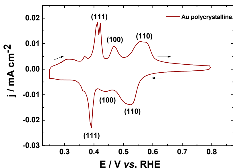
Figure 7. Cyclic voltammogram of Au polycrystalline in 0.1 \text{ mol L}^{-1} \text{ NaOH} + 1 \text{ mmol L}^{-1} \text{ Pb}(\text{NO}_3)_2 , recorded at 20 \text{ mV s}^{-1} and at 20 \text{ }^\circ\text{C} .
