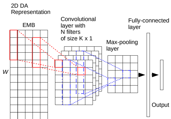
Figure 1: CNN_1 architecture
