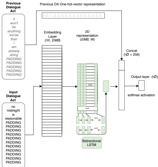
Figure 2: Bidirectional LSTM architecture
