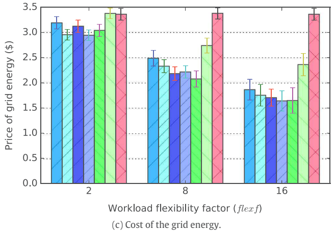
Fig. 11. Comparison of the results between the approaches and heuristics, for workloads with different flexibility values. The standard deviation is represented, as each experiment is repeated with 10 workloads generated using different random seeds.
