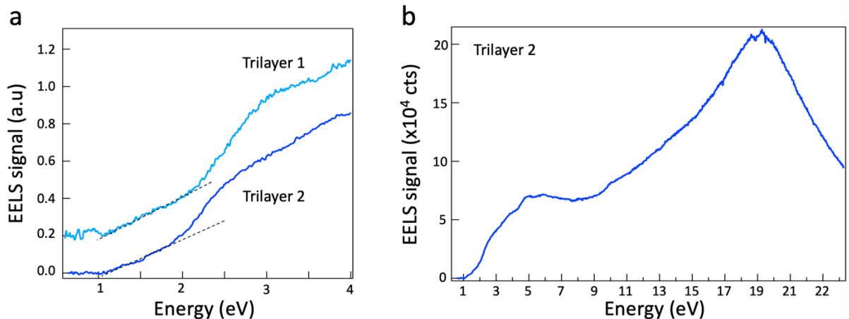
Figure S3. a EELS spectrum of trilayer 1 and trilayer 2 shown in Figures S1 and S2. from 0.6 eV to 4 eV. b EELS spectra of trilayer 2 recorded at 80kV from 0.6 eV to 22 eV. Spectra recorded at 80kV.
