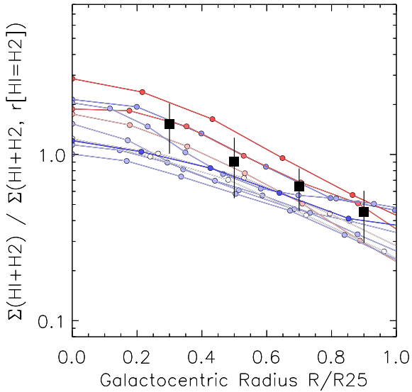
Figure 4. Total gas profiles (H I + H 2 ) of the 11 BLUEDISK galaxies with reliable profiles, normalized to the surface density at the transition radius (where \Sigma_{\text{H I}} = \Sigma_{\text{H}_2} ). Same colour-coding as in Fig. 1. The mean values found by Bigiel & Blitz (2012) in nearby, late-type discs are overplotted as black squares.
