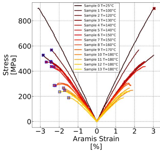
Fig. 6. High temperature Flexion tests results
